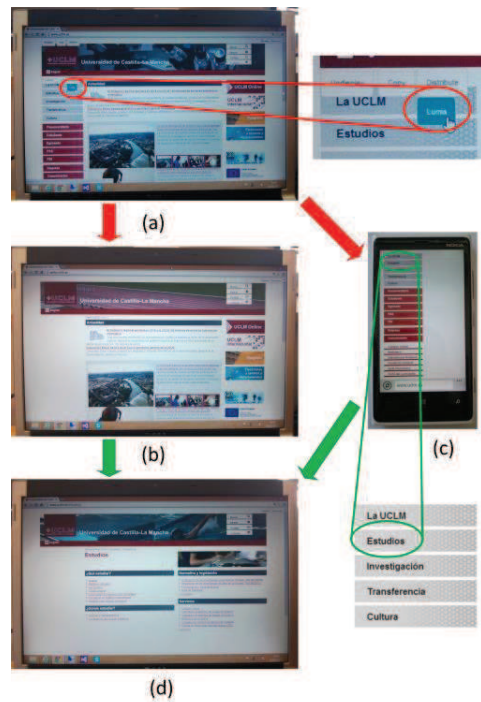
Figure 2. Distributing the navigation menu
