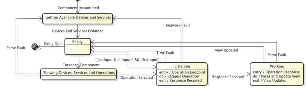
Figure 5. Generic State Diagram for DUI Components.
