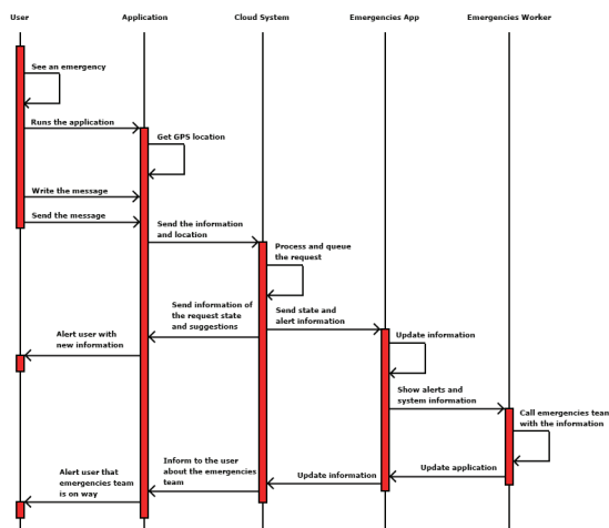
Figure 1: Ideal sequence diagram in the process
