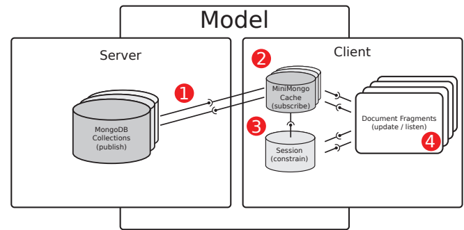
Figure 2. Conceptual Data Model using Meteor.
