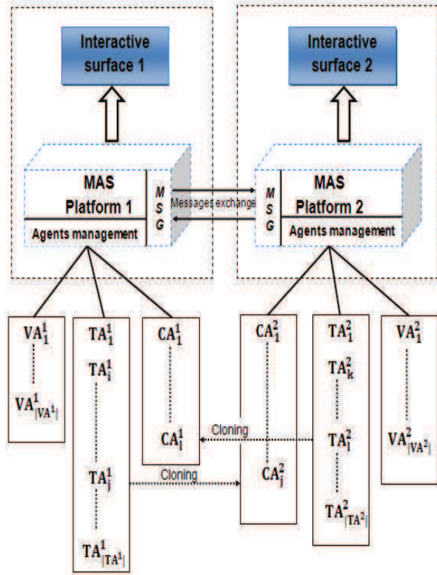
Figure 1. Model dedicated to the management of distributed interactive surfaces with MAS Platforms (legend: TA = Tangiget Agent; VA = Virtual Agent; CA = Clone Agent, MSG = messages protocols)
