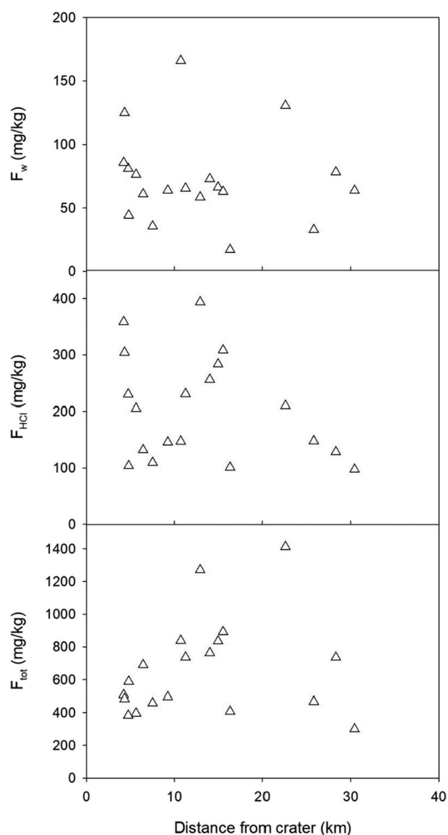
Fig. 3 Concentrations of water-extractable fluoride ( F_w ), HCl-extractable fluoride ( F_{HCl} ), and total fluoride ( F_{tot} ) in the soil samples versus distance from Masaya Volcano's degassing crater
