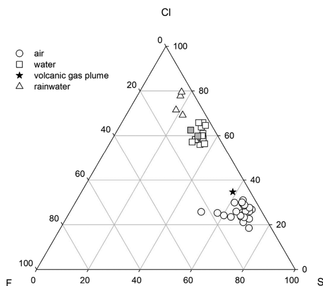
Fig. 6 Relative molar concentrations of sulfur, chlorine and fluorine in air, water, volcanic gas plume and rainwater samples. The two grey-filled squares represent the non-drinking water samples. See text for explanations
