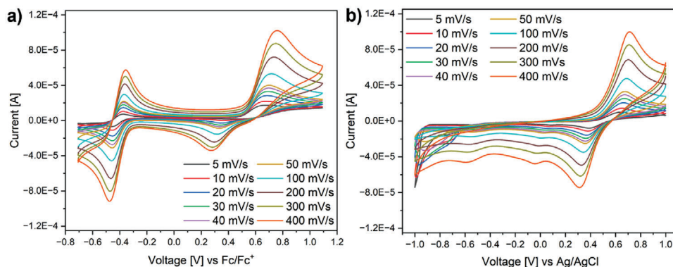
Figure 7. a) Cyclic voltammograms of [\text{C}_4\text{py}][\text{FeCl}_4] in a solution of 100 mM TBAP (tetrabutylammonium perchlorate) in MeCN; b) Cyclic voltammograms of [\text{C}_4\text{py}][\text{FeCl}_4] in a solution of 1000 mM \text{KNO}_3 in \text{H}_2\text{O} .
