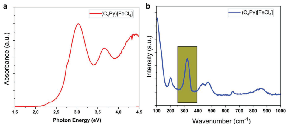
Figure 6. a) Solid-state absorption spectra of [\text{C}_4\text{py}][\text{FeCl}_4] at room temperature. The data have been acquired through UV reflectance measurements. b) Raman spectrum of [\text{C}_4\text{py}][\text{FeCl}_4] with the A1 mode highlighted in gold.
