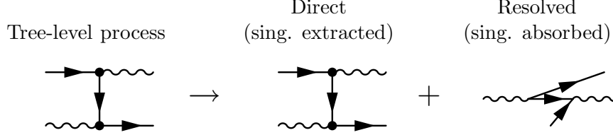
Figure 1.18: Illustration of the singularity extraction for the W + \text{quark} photoproduction.
