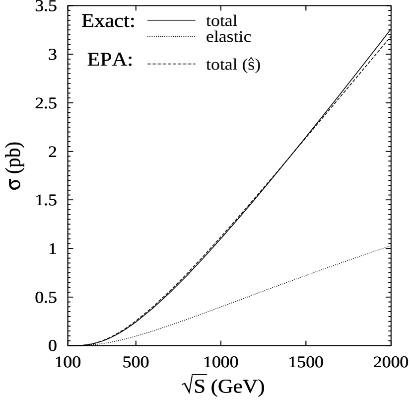
Figure 1.11: Comparison of exact computation of the process ep \rightarrow \nu W X with the result obtained through EPA. The EPA elastic component is indistinguishable from the exact calculation
