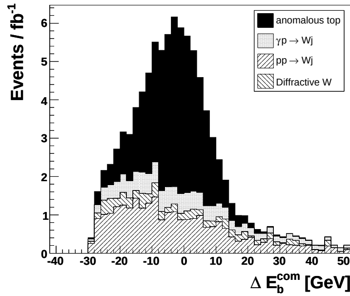
Figure 4.19: Distribution of the b-jet energy the centre of mass frame of the top quark, reconstructed using the photon energy information from very forward detectors. Basic acceptance cuts, exclusivity condition, b-tagging and proton tag were required
