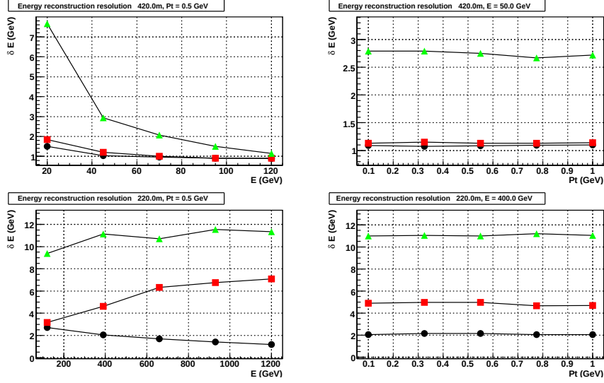
Figure 3.13: Resolution of the reconstructed energy loss of protons as a function of the energy loss (left) and the transverses momentum (right), for stations at 420 m (up) and 220 m (down). The detector resolution was supposed to be perfect (no smearing, circles), 5 \mu\text{m} (squares) and 30 \mu\text{m} (triangles).
