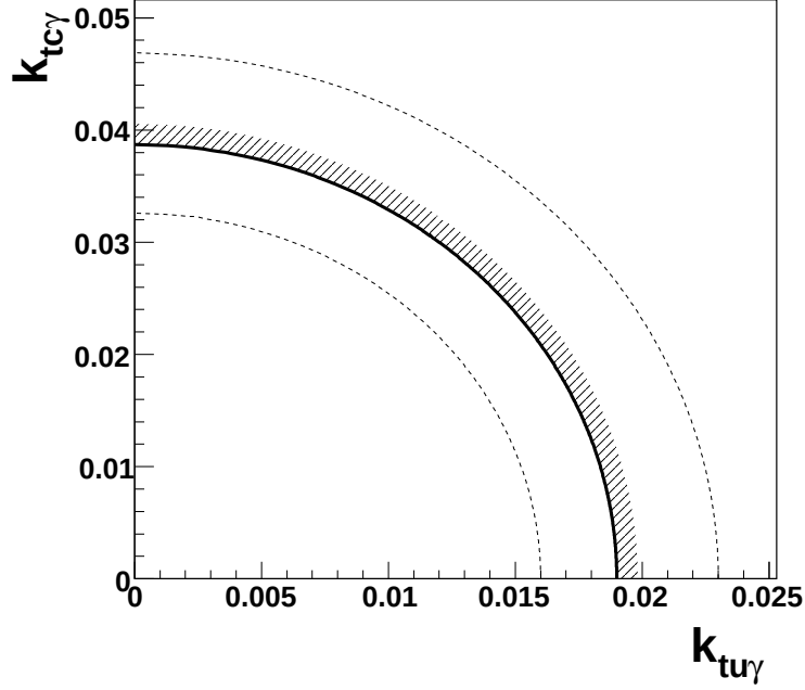
Figure 4.22: Two-dimensional limits on the anomalous couplings k_{tu\gamma} and k_{tc\gamma} (solid) for the intermediate scenario of an instantaneous luminosity of 2 \times 10^{33} \text{cm}^{-2} \text{s}^{-1} and 30 \text{fb}^{-1} of integrated luminosity using VFDs for tagging and reconstruction. The other lines correspond to a positive or negative variation of the observed number according to the systematic uncertainty.
