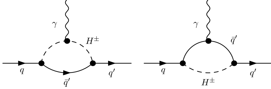
Figure 1.20: One-loop diagrams for FCNC in Multi-Higgs Models
