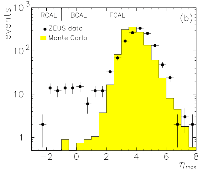
Figure 1.4: Number of observed events as a function of the pseudo-rapidity \eta_{\max} of the most forward calorimeter cluster in the ZEUS detector, compared with the Monte Carlo DIS expectation. One clearly sees the excess of events with an important rapidity gap between the outgoing proton direction and any activity in the detector [17].
