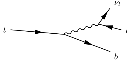
Figure 4.6: Top SM decay into a jet, a charged lepton and a neutrino
