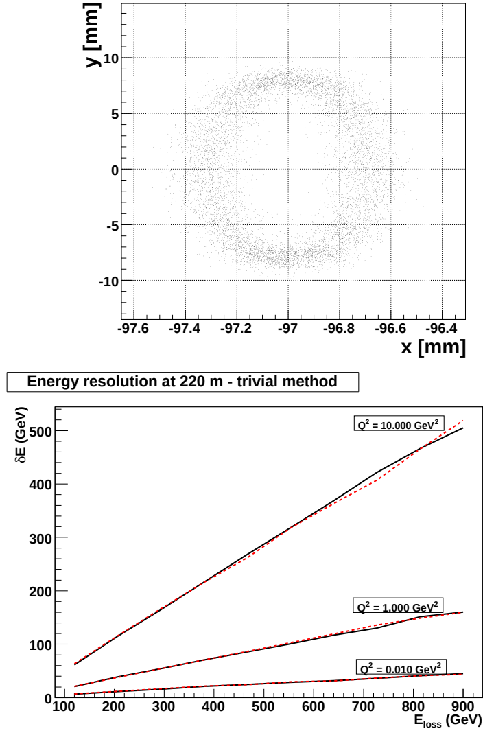
Figure 3.11: Effect of momentum transfer of 10 \text{ GeV}^2 on the beam profile (left). As the position is measured only using one detector plane, this affects strongly the reconstructed energy resolution (right).
