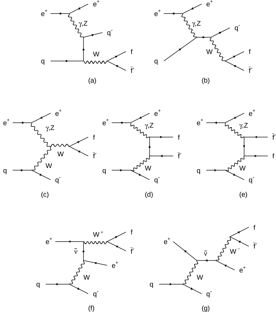
Figure 2.1: Diagrams for W boson production in the Standard Model with the subsequent decay to fermions. The process ep \rightarrow \nu_e W X is not depicted. Diagram (c) is sensitive to possible anomalous triple gauge couplings. Diagrams (d) and (e) are included to preserve gauge invariance. The present analysis only focuses on final states including an electron and a neutrino.
