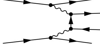
Figure 1.10: Lepton pair production via photon-photon interaction
