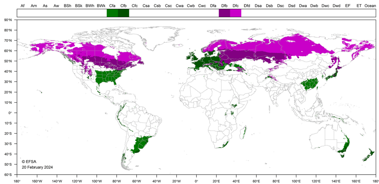
FIGURE 2 World distribution of Köppen–Geiger climate types that occur in the EU and which occur in countries where Crisicoccus seruratus has been reported.
