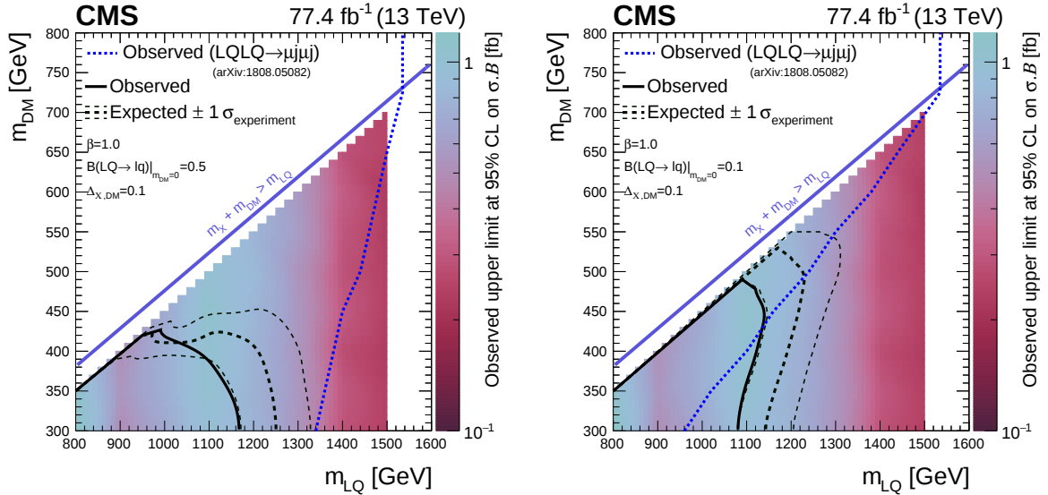
Figure 4: Observed 95% CL upper limits on the product of cross section and branching fraction for the signal model of Fig. 1 assuming \mathcal{B}(LQ \rightarrow c\mu) to be (left) 0.5 or (right) 0.1. The solid and dashed (black) curves show the observed and expected 95% CL exclusion curves. The dotted (blue) curve shows the corresponding observed limits from the recast of the results from a search for pair produced second-generation LQs [20].
