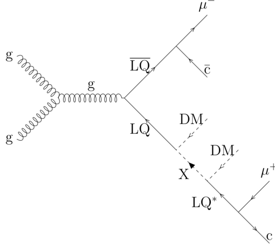
Figure 1: An example Feynman diagram for the signal process considered in this study, where g is a gluon, LQ a leptoquark, DM a dark matter particle, and X a new Dirac fermion. The superscript “*” indicates an off-shell particle.
