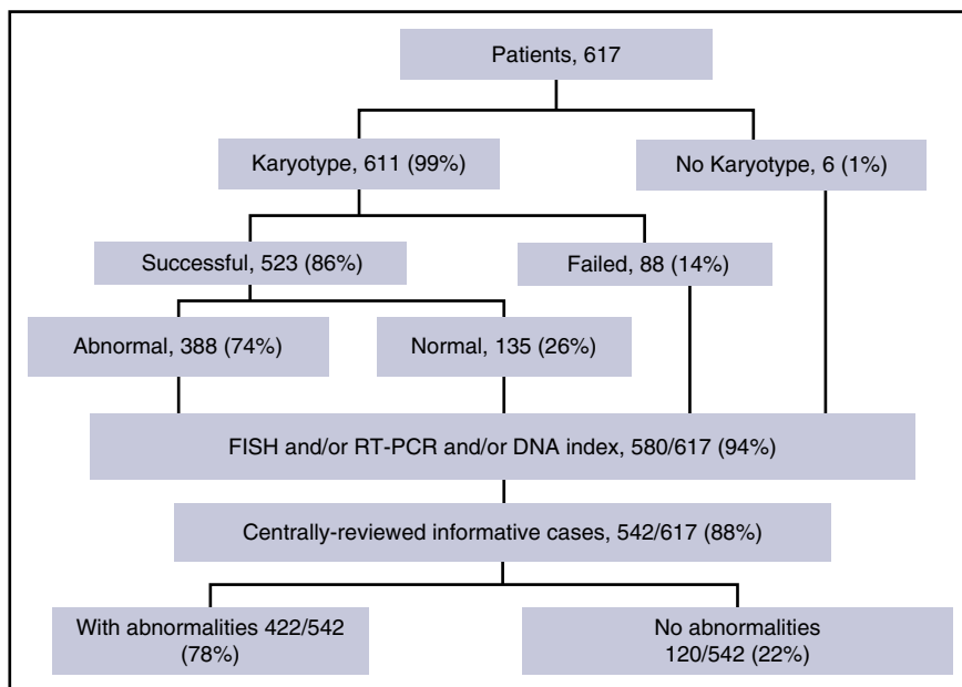
Figure 1. Cytogenetic flowchart.
