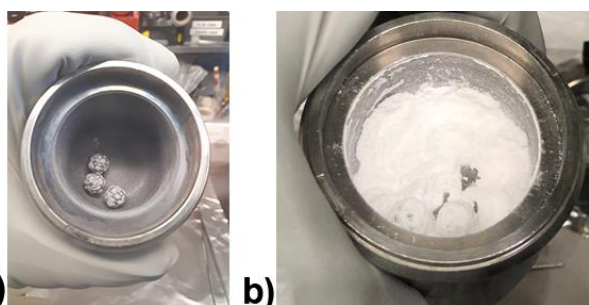
Figure 6. Photo of stainless-steel jar after ball-milling of [\text{Mg(en)}_3(\text{BH}_4)_2] : \text{Mg}(\text{BH}_4)_2 = 3 : 2 at room temperature at BPR = 60:1 (left) and in jar pre-cooled by ^i\text{PrOH} -liquid \text{N}_2 at BPR = 60:1 (right).
