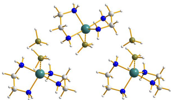
Figure 5. A fragment of the crystal structure of \text{Mg}(\text{en})_2(\text{BH}_4)_2 . Colour scheme: Mg (aquamarine), N (blue), B (olive), C (grey), H (dark grey).
