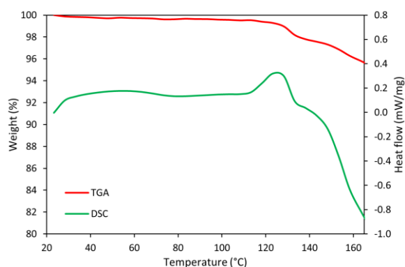
Figure 2. TGA-DSC curves for the \text{Mg}(\text{en})_{1.2}(\text{BH}_4)_2 sample prepared according to Scheme 1 (a). The endothermic decomposition occurs with concomitant weight loss at 123°C.
