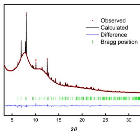
Figure 7. Rietveld refinement of the \text{Mg(en)}_2(\text{BH}_4)_2 crystal phase. The powder pattern was measured at SNBL/ESRF with a wavelength of 0.77936 Å. R_B = 14.5\% (space group P2_12_12_1 , a = 9.3580(4) , b = 8.8374(4) , c = 7.1311(3) Å), R_{wp} = 0.766 , \chi^2 = 20 .
