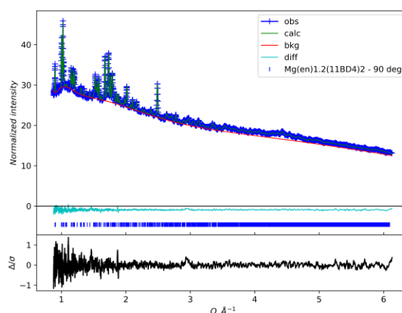
Figure 4. Rietveld refinement profile for the NPD pattern of \text{Mg}(\text{en})_{1.2}(^{11}\text{BD}_4)_2 using the structural model obtained from single crystal synchrotron X-ray diffraction. Data were collected at the NOVA beamline at J-PARC, Japan. The sample was labelled with ^{11}\text{B} instead of natural B and deuterium on the borohydride but not on the en ligand.
