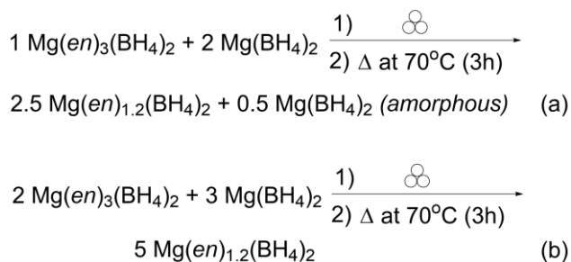
Scheme 1. Synthesis of \text{Mg}(\text{en})_{1.2}(\text{BH}_4)_2 by ball-milling with subsequent annealing.
