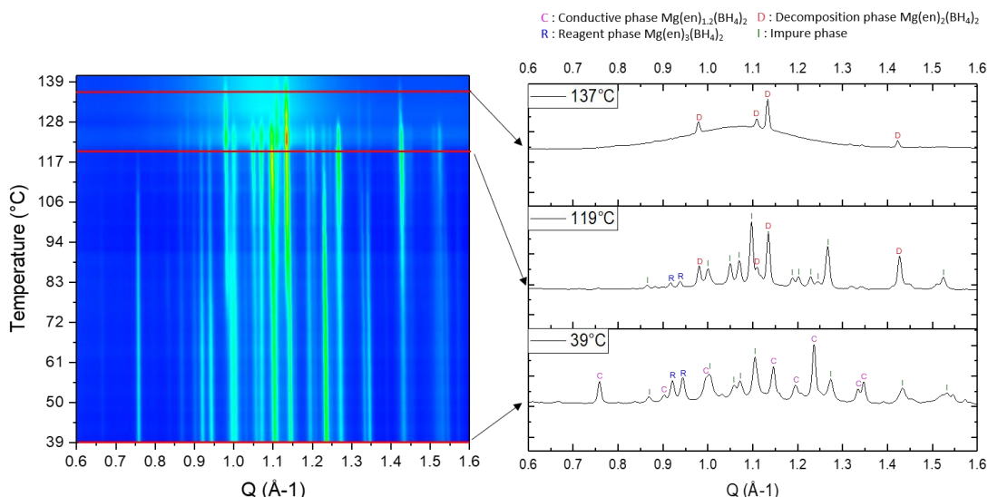
Figure 1. In situ SR-XRPD vs temperature for “ \text{Mg}(\text{en})_1(\text{BH}_4)_2 ” prepared by Scheme 1 (a). Besides the main \text{Mg}(\text{en})_{1.2}(\text{BH}_4)_2 phase (C), two side products are observed: an impurity (I) and the decomposition (D) phases. Small amounts of reagents (R) typically remain in the samples. Upon heating, first the \text{Mg}(\text{en})_{1.2}(\text{BH}_4)_2 phase decomposes, at higher temperatures only the D phase remains crystalline.
