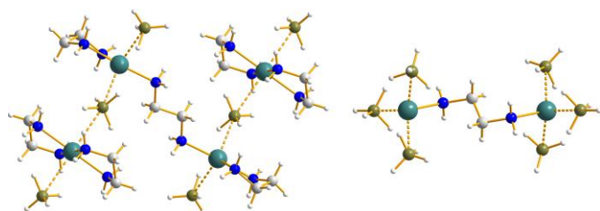
Figure 3. The crystal structure of \text{Mg}(\text{en})_{1.2}(\text{BH}_4)_2 : the cation [\text{Mg}_3(\text{en})_5(\text{BH}_4)_4]^{2+} constituting the coordination polymer chains [\text{Mg}^{2+}(\kappa^2\text{-en})_2(\mu_2\kappa^{1,2}:\kappa^2\text{-BH}_4^-)\text{Mg}^{2+}(\kappa^2\text{-en})(\kappa^2\text{-BH}_4^-)(\mu_2\text{-en})\text{Mg}^{2+}(\kappa^2\text{-en})(\kappa^2\text{-BH}_4^-)(\mu_2\kappa^{1,2}:\kappa^2\text{-BH}_4^-)] (left) and the isolated binuclear anion [\{\text{Mg}(\kappa^3\text{-BH}_4)(\kappa^2\text{-BH}_4)_2(\mu_2\text{-en})\}^{2-}] (right). Colour scheme: Mg (aquamarine), N (blue), B (olive), C (grey), H (white).
