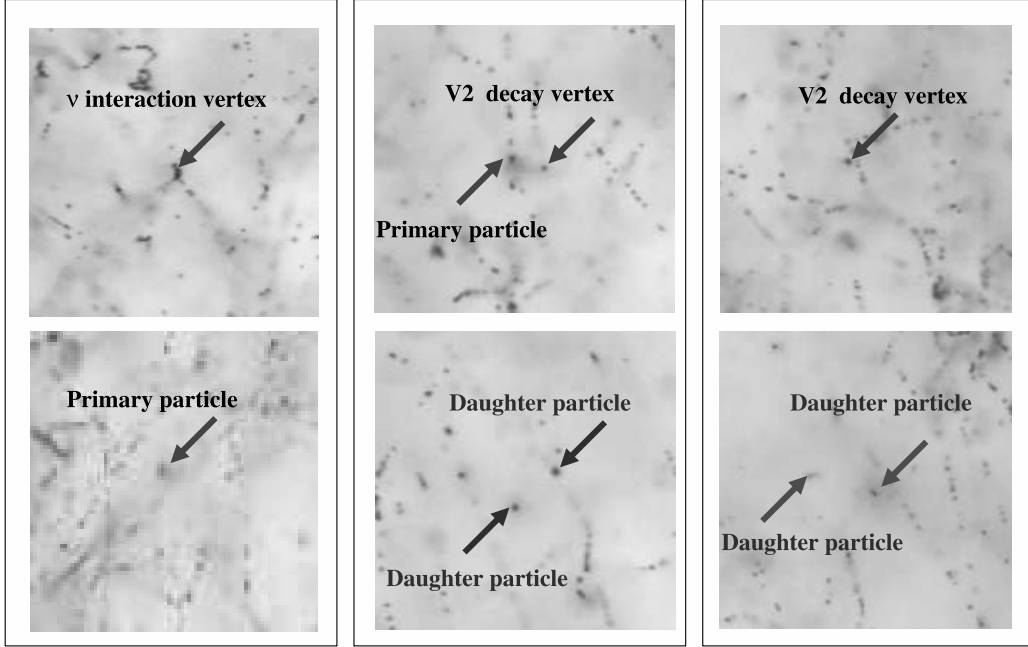
Figure 3: Microscope views of Event 8132-12312 taken in the emulsion. Since the neutrino beam is perpendicular to the emulsion target, the trajectory of a charged particle appears as a 'dot'. The top-left picture shows the neutrino interaction vertex. A charged particle which is visible several microns downstream of the vertex emerges from the neutrino vertex. The top-center picture shows the decay vertex of a neutral charmed particle decaying into two charged particles (V2) 63 \mu\text{m} downstream of the primary vertex. The trajectory of the daughter particles is visible at bottom-center picture. A second V2 decay topology is found 977 \mu\text{m} downstream of the primary vertex as shown in the top-right picture. In the bottom-right picture the trajectory of daughter particles from the second neutral decay becomes visible after several microns downstream of the decay vertex.
