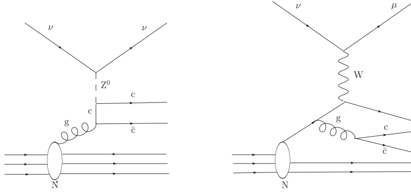
Figure 1: Feynman diagrams for boson-gluon fusion(left) and gluon bremsstrahlung processes(right).
