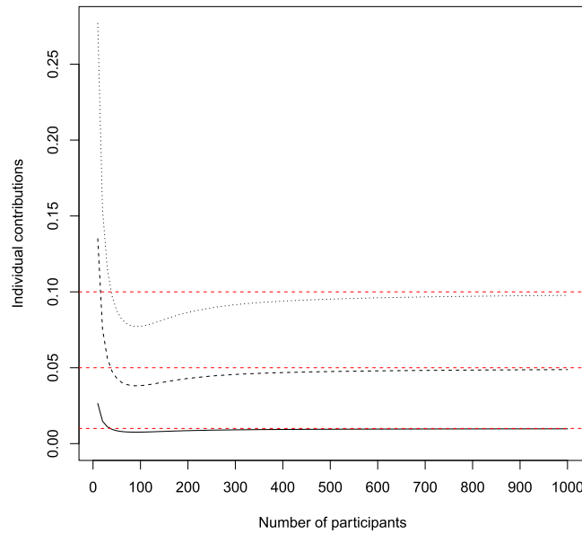
Fig. 1. Individual contributions c_{i,n}^{\text{uni}} in function of the number n of participants to the endowment contingency fund, for participant i in Group 1 (solid line, —), in Group 2 (broken line, - - -), and in Group 3 (dotted line, ...). Red horizontal lines corresponding to respective occurrence probabilities.
