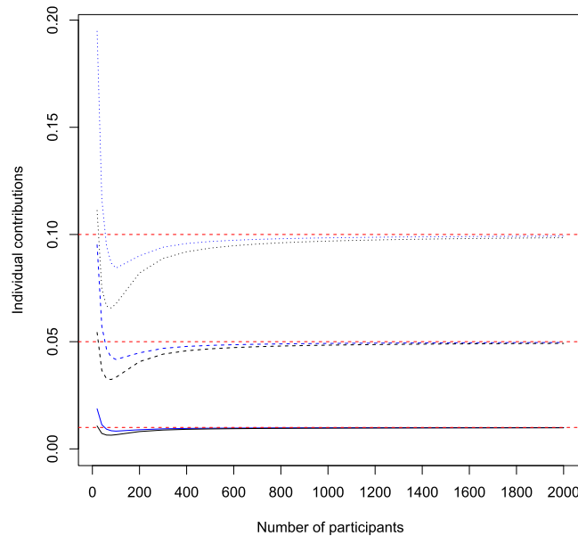
Fig. 3. Individual contributions per unit in Group 1 (solid line, —), in Group 2 (broken line, - - -), and in Group 3 (dotted line, ...), blue curves correspond to participants with w_i = 1 and black curves to participants with w_i = 2 , with red horizontal lines at occurrence probabilities.
