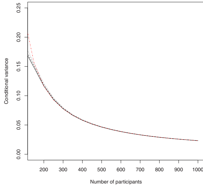
Fig. 2. Conditional variance \text{Var}[T_{i,n}^{\text{uni}} | I_i = 1] in function of the number n of participants to the endowment contingency fund, for participant i in Group 1 (solid line, —), in Group 2 (broken line, - - -), and in Group 3 (dotted line, ...). Red curve corresponding to the approximation deduced from Proposition 3.
