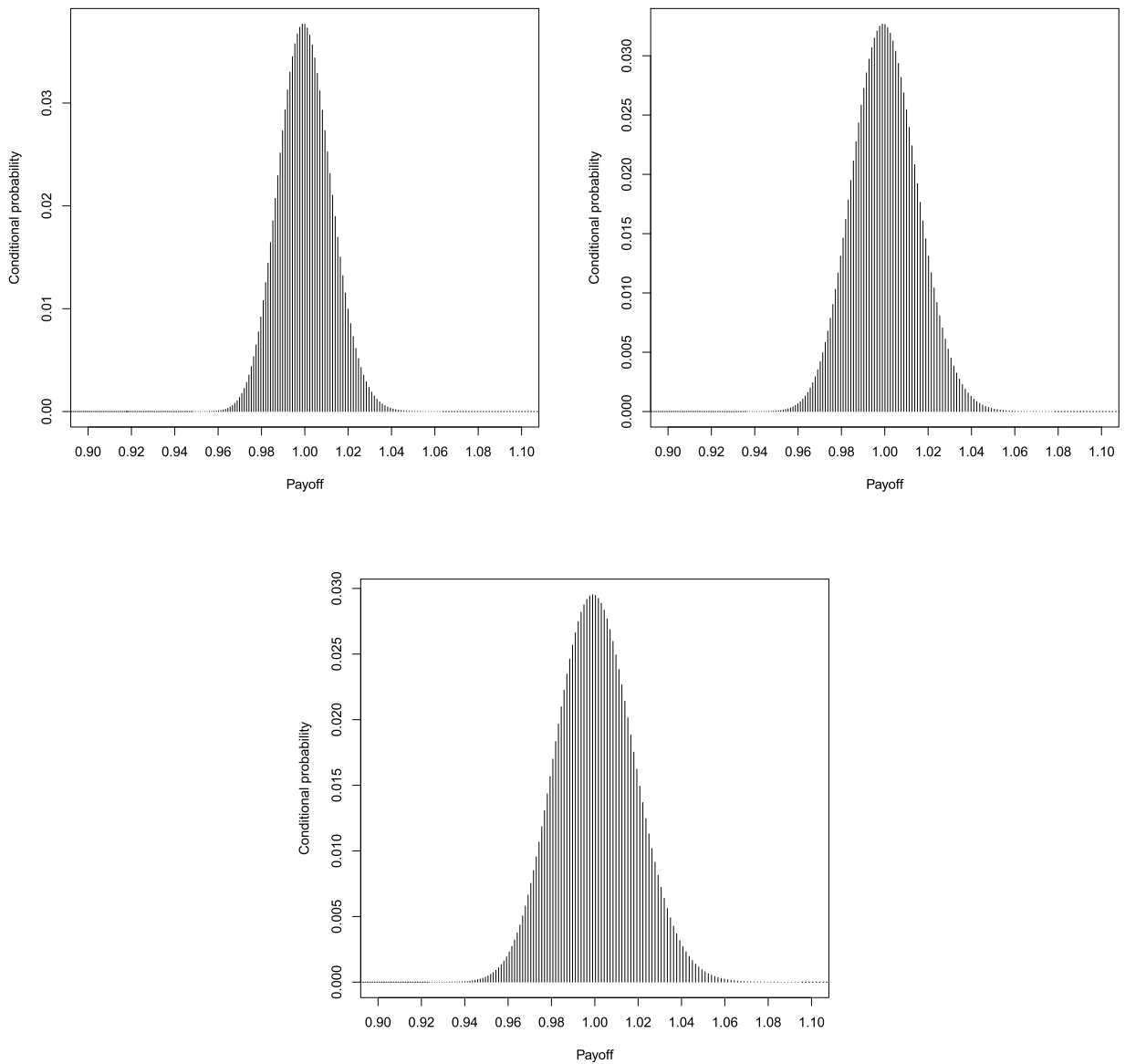
Fig. 5. Probability mass function of the terminal payoff to a survivor for an endowment longevity fund gathering n = 1,000 participants with uniform protection level. Results corresponding to a participant aged 65 at policy issue, for payments at time 6 (upper left panel), 8 (upper right panel), and 10 (lower panel).
