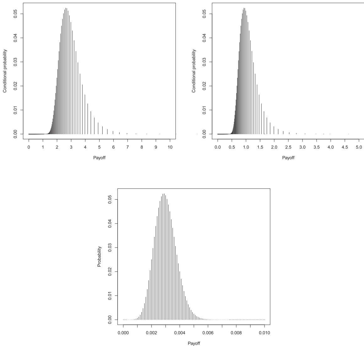
Fig. 4. Probability mass function of the terminal payoff to a claiming participant aged up to 39 (upper left panel), aged 40–59 (upper right panel), and probability mass function of the share of total losses under XHB system (bottom panel) for n = 10,000 participants.
