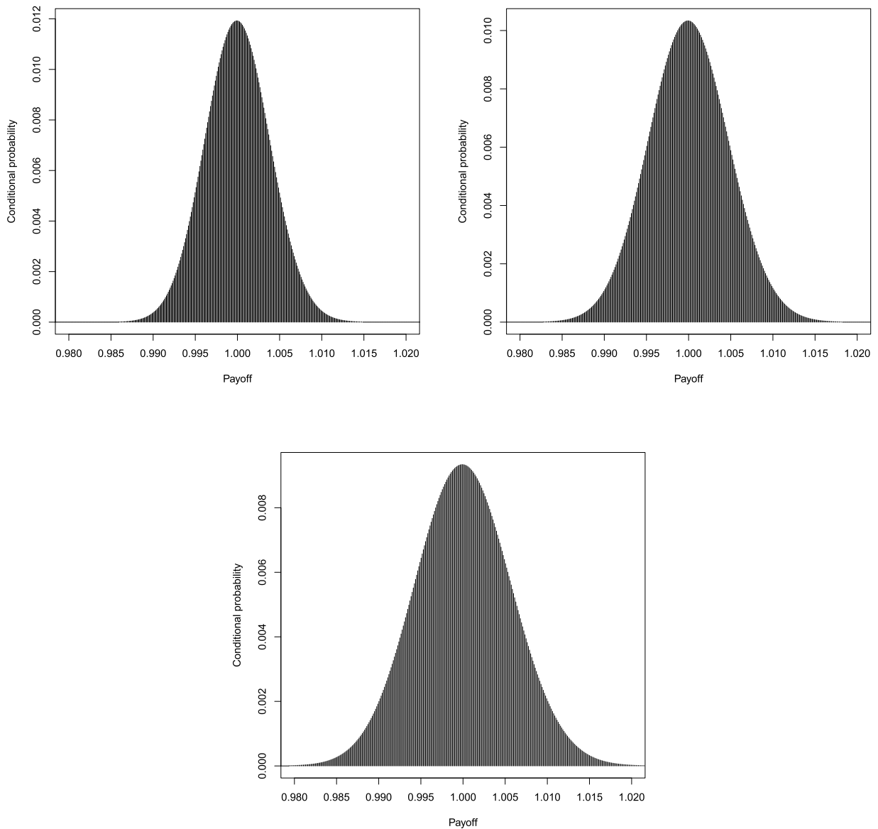
Fig. 6. Probability mass function of the terminal payoff to a survivor for an endowment longevity fund gathering n = 10,000 participants with uniform protection level. Results corresponding to a participant aged 65 at policy issue, for payments at time 6 (upper left panel), 8 (upper right panel), and 10 (lower panel).
