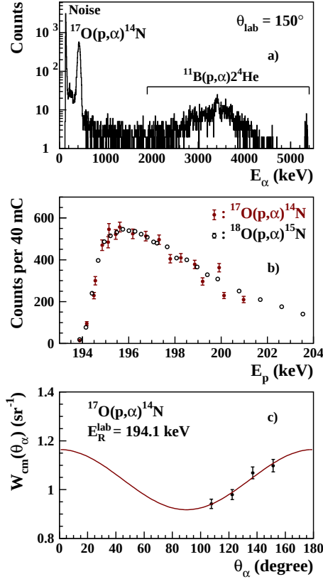
FIG. 2: (a) Sample \alpha spectrum obtained in the ^{17}\text{O}(p,\alpha)^{14}\text{N} experiment, for E_p=196.5 keV and an accumulated charge of 0.93 C. (b) Yield data for the new resonance at E_R^{\text{lab}}=194.1 keV in the ^{17}\text{O}(p,\alpha)^{14}\text{N} reaction (filled symbols) and the well-known ^{18}\text{O}(p,\alpha)^{15}\text{N} resonance at E_R^{\text{lab}}=150.9 keV (empty symbols). The data for this latter resonance were appropriately normalized and shifted in energy to be compared with those obtained with the ^{17}\text{O} target. (c) \alpha angular distribution (center-of-mass) for the ^{17}\text{O}(p,\alpha)^{14}\text{N} resonance. The solid line shows a Legendre-polynomial fit to the data, W_{\text{cm}}(\theta_\alpha) = 1 + a_2 P_2(\cos\theta_\alpha) , which yields a_2=0.16\pm0.03 .
