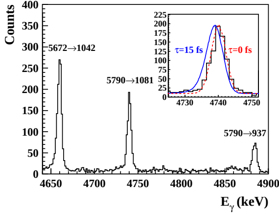
FIG. 1: Relevant part of a sample \gamma -ray spectrum obtained in the ^{14}\text{N}(\alpha, \gamma)^{18}\text{F} experiment with the Ge detector at \theta_{lab}=0^\circ . The inset shows a comparison of the observed full-energy peak for the 5789.8→1080.54 keV transition in ^{18}\text{F} with simulated line emissions calculated for a mean lifetime \tau of the 5789.8 keV state equal to 15 fs (solid curve) and 0 fs (dashed curve).
