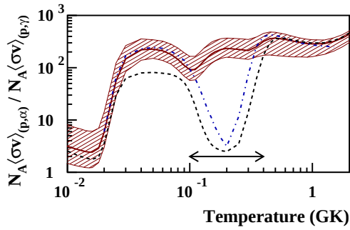
FIG. 4: Ratio of the ^{17}\text{O}(p,\alpha)^{14}\text{N} and ^{17}\text{O}(p,\gamma)^{18}\text{F} reaction rates (solid line with hatched area reflecting uncertainties), in comparison with the previous results of Angulo et al. [8] (dashed line) and Fox et al. [5] (dotted-dashed line). The horizontal arrow shows the range of typical novae temperatures.
