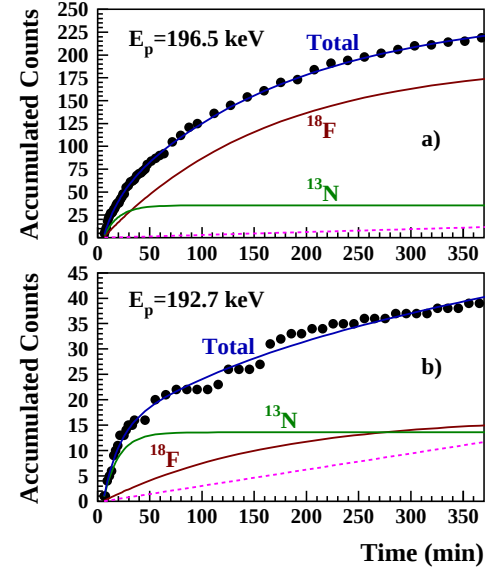
FIG. 3: Measured \beta^+ activities of two ^{17}\text{O} -implanted targets irradiated at (a) E_p=196.5 keV (on-resonance) and (b) E_p=192.7 keV (off-resonance). The time origin corresponds to the stopping of the proton irradiation. Also shown are the fitted ^{18}\text{F} and ^{13}\text{N} decay curves (solid lines) and the measured background radiation (dashed lines).
