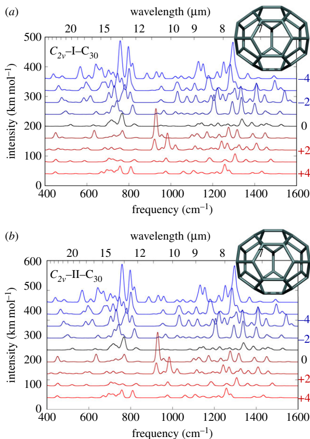
Figure 12. Two principal classical fullerene isomers of C_{30} : (a) C_{2v}-I-C_{30} and (b) C_{2v}-II-C_{30} . Isomer structures and calculated IR spectra in cm^{-1} in various charge states, as marked. (Online version in colour.)
