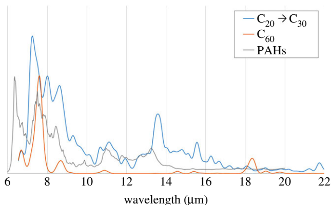
Figure 15. Sum of all 478 purely carbon–hydrogen species in the NASA AMES PAH database. Each spectrum intensity is divided by the number of carbon atoms in the PAH (convolved with a Lorentzian emission profile with a FWHM of 10\text{ cm}^{-1} ). As can be seen, in good agreement with literature reports of PAH interstellar bands, there is strong absorption across the 6\text{--}9\text{ }\mu\text{m} range, with secondary features in the 10\text{--}14\text{ }\mu\text{m} region, and relatively little signal in the 14\text{--}20\text{ }\mu\text{m} range. In comparison, similarly weighted sums of all small fullerene and \text{C}_{60} calculations in this paper notably show extensive fullerene cage modes in the 14\text{--}18\text{ }\mu\text{m} range.
