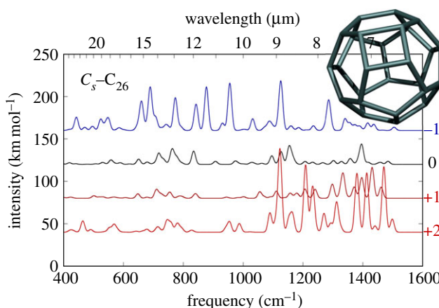
Figure 8. Calculated IR spectra for C_s\text{-C}_{26} ( \text{cm}^{-1} ) in various charge states, as marked. (Online version in colour.)
