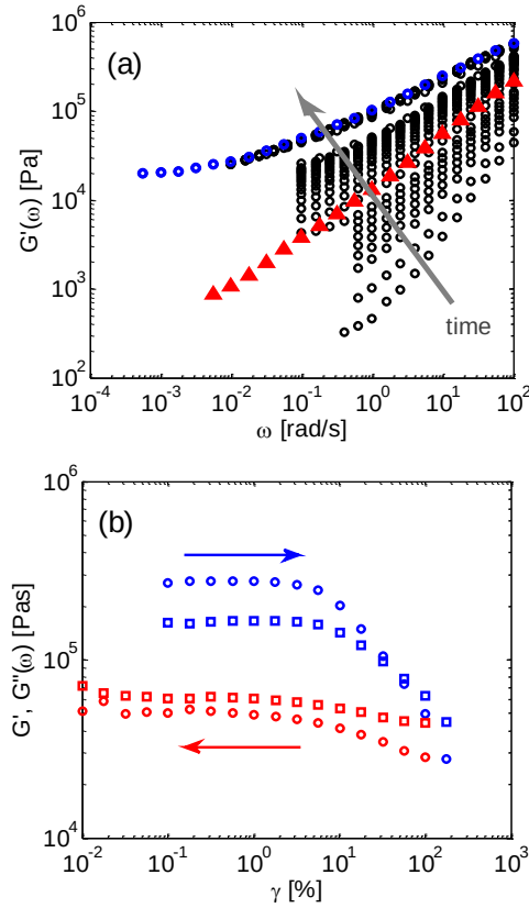
Figure 3.7: (a) Evolution through time of the storage modulus of the metallo-supramolecular systems obtained by adding 0.75 eq. of nickel ions to the bi-functional PEO building blocks (black ○), toward its equilibrium state (blue ○). The data represented by the triangle symbols have been measured right after the strain sweep measurements (see Figure b), and show the partial breaking of the supramolecular network. (b): Storage (○) and loss (□) moduli of the same sample, measured as a function of the amplitude of deformation, at a freq. of 10 rad/s. First from low to high, then from high to low amplitude of deformation.
