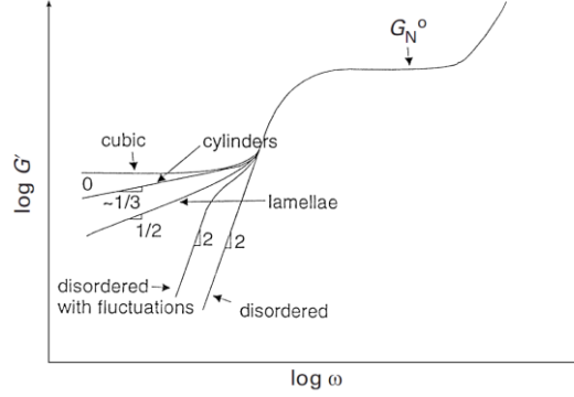
Figure 2.2: Schematic representation of the linear viscoelastic response of diblock copolymers with various equilibrium and non-equilibrium long range ordering structures. Adopted from Kossuth et al. J. Rheol. 1999. 4
