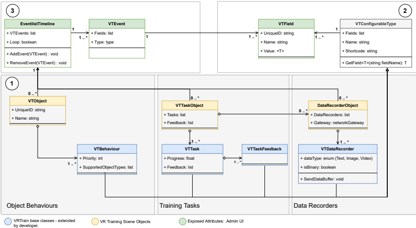
Fig. 7. VRTrain Event Dispatcher Class Diagram.
