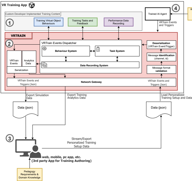
Fig. 8. VR Training Simulation: Development and Authoring with VRTrain.
