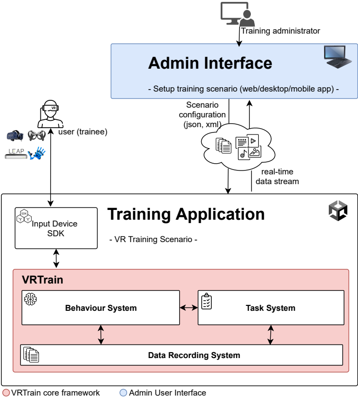
Fig. 6. VRTrain Architecture
