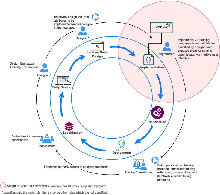
Fig. 4. VRTrain framework: target users and context of use.
