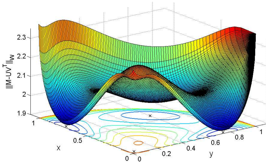
FIG. 2.1. Objective function of (WLRA) with respect to the parameters (x, y) .
