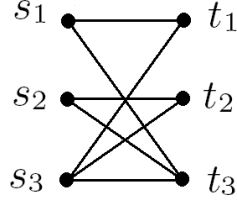
FIG. 3.1. Graph corresponding to the matrix M of Example 1.
