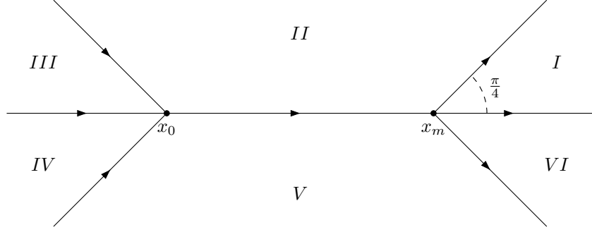
Figure 3: Jump contours \Sigma_{\sin} for the RH problem for \Phi_{\sin} .
