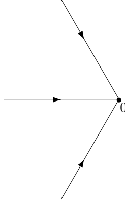
Figure 8: The jump contour \Sigma_{\text{Be}} for \Phi_{\text{Be}} .
