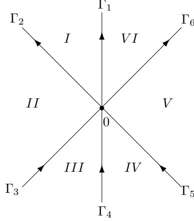
Figure 9: The jump contour \Sigma_{\text{HG}} for \Phi_{\text{HG}} . The ray \Gamma_k is oriented from 0 to \infty , and forms an angle with \mathbb{R}^+ which is a multiple of \frac{\pi}{4} .
