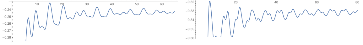
Figure 1: Numerical confirmations of Theorem 1.1.
