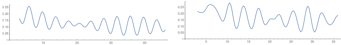
Figure 2: Numerical confirmations of Theorem 1.2.
