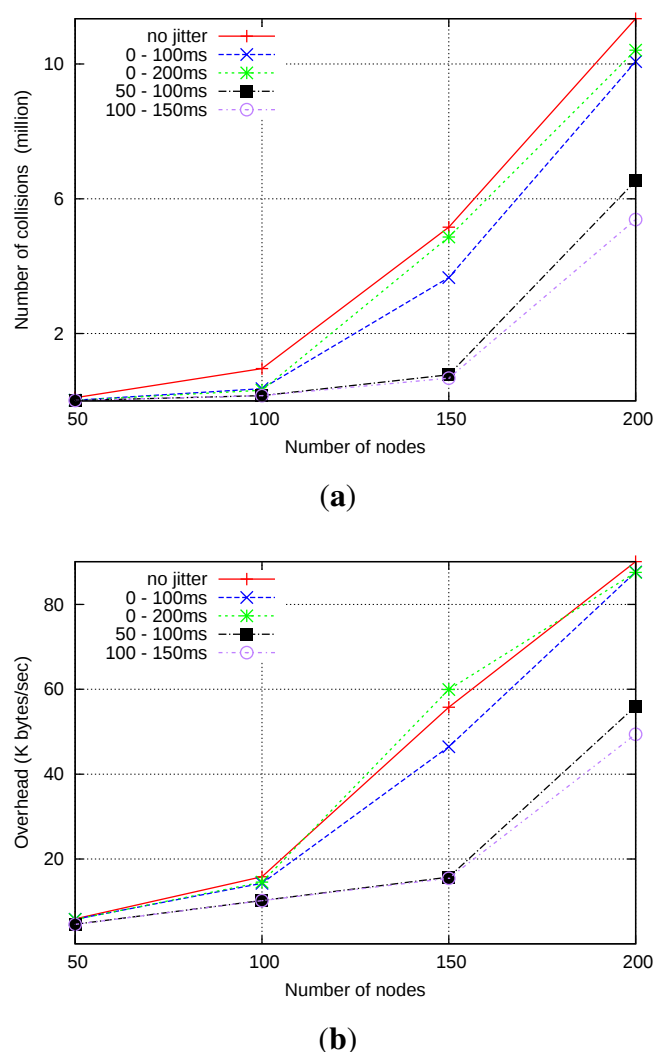
Figure 16. Simulation results of shortest-path RREQ forwarding. (a) Number of collisions; (b) Average overhead.
