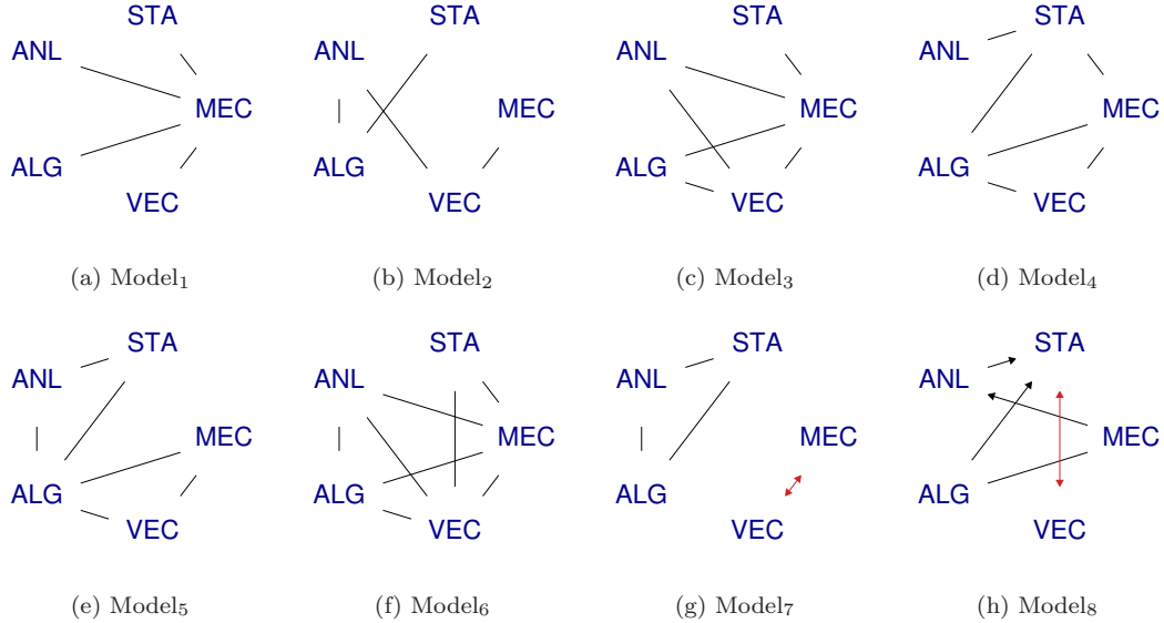
Fig. 7: Mathematics grades. Eight candidate models, from which selection of the best model takes place.
