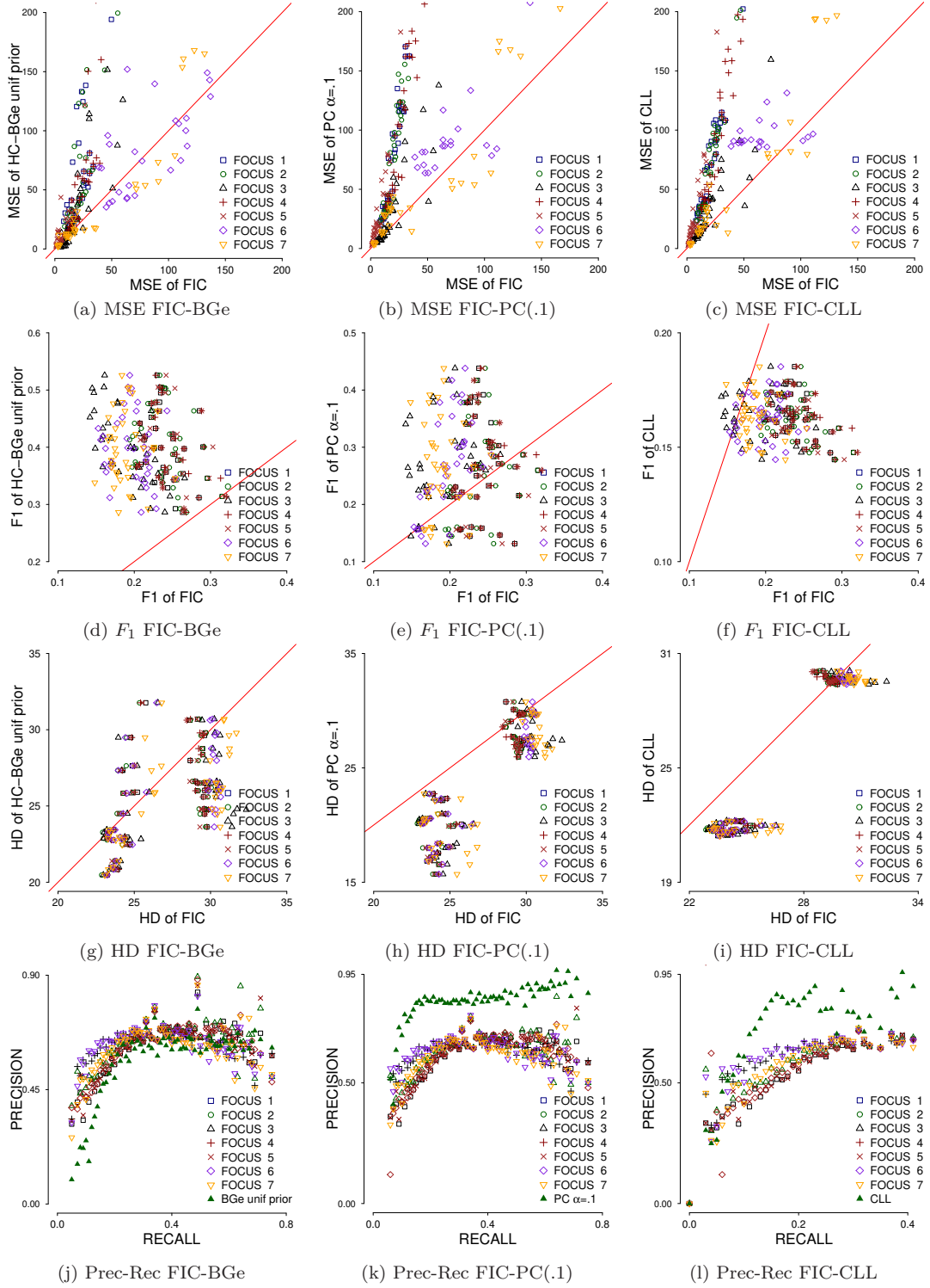
Fig. 4: Empirical MSE (a-c), F_1 index (d-f), Hamming distance (g-i) and precision-recall plots (j-l) of FIC plotted against the performance of competitor methods for 7 focus values and 36 simulation settings, averaged over 500 simulation runs for networks with 10 nodes. Random errors are generated from a multivariate t(10) distribution.
