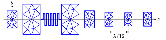
Fig. 7. Meshed patches used for implementing one 2\lambda/3 period of the MTS (along x ): rectangular patches (capacitive) and meander lines (inductive) of varying sizes.
