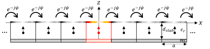
Fig. 2. 1-D infinite periodic MTS antenna, where the reference cell and the corresponding reference feed are highlighted in red.
