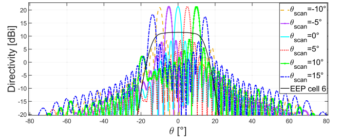
Fig. 10. MTS array pattern for various scanning directions \theta_{scan} , for an antenna of length 22\lambda (11 cells) with four subfeeds per cell.
