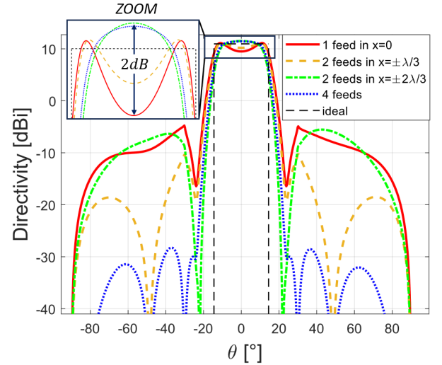
Fig. 6. EEP directivity for different feed configurations: one unitary feed located at x = 0 , two unitary subfeeds located at x = \pm\lambda/3 and x = \pm2\lambda/3 , and four subfeeds of amplitudes A = [0.5, 1, 1, 0.5] located at x = [-\lambda, -\lambda/3, \lambda/3, \lambda] .
