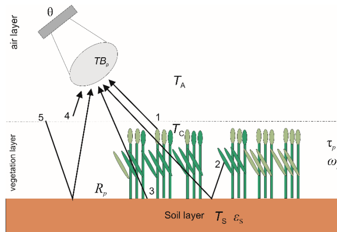
Figure 2. Schematic view of the \tau - \omega model used to describe the different contributions of the brightness temperature measured by a radiometer antenna at a specific incidence angle ( \theta ). Here, a soil layer with a temperature T_S is covered by a vegetation layer with a temperature T_C and an air layer characterized by a temperature T_A . The soil is also characterized by a soil surface reflectivity ( R_p ) and a soil relative dielectric permittivity ( \epsilon_s ), while the vegetation is characterized by an effective scattering albedo ( \omega_p ) and a vegetation optical depth ( \tau_p ). Both vegetation parameters can be defined as polarization (indices p ) dependent (adapted from Mo et al. [12] and Vereecken et al. [4]).
