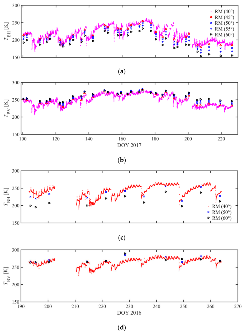
Figure 6. Brightness temperature ( T_B ) measured for of the non-gridded plot covered by wheat vegetation at different incidence angles from 40° to 60° measured in 5° increments for H polarization (a) and V polarization (b). T_B measurements for the non-gridded plot covered by mustard vegetation considering also incidence angles from 40° to 60°, but with 10° increments for H polarization (c) and V polarization (d).
