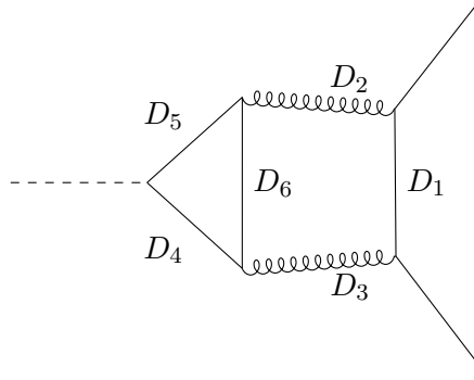
Figure 4.7: Correspondence between the denominators for our topology and the denominator in one of our Feynman diagrams.
