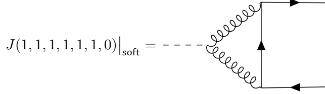
Figure 4.8: Diagrammatic interpretation of the soft contribution to the integral J(1, 1, 1, 1, 1, 0)
