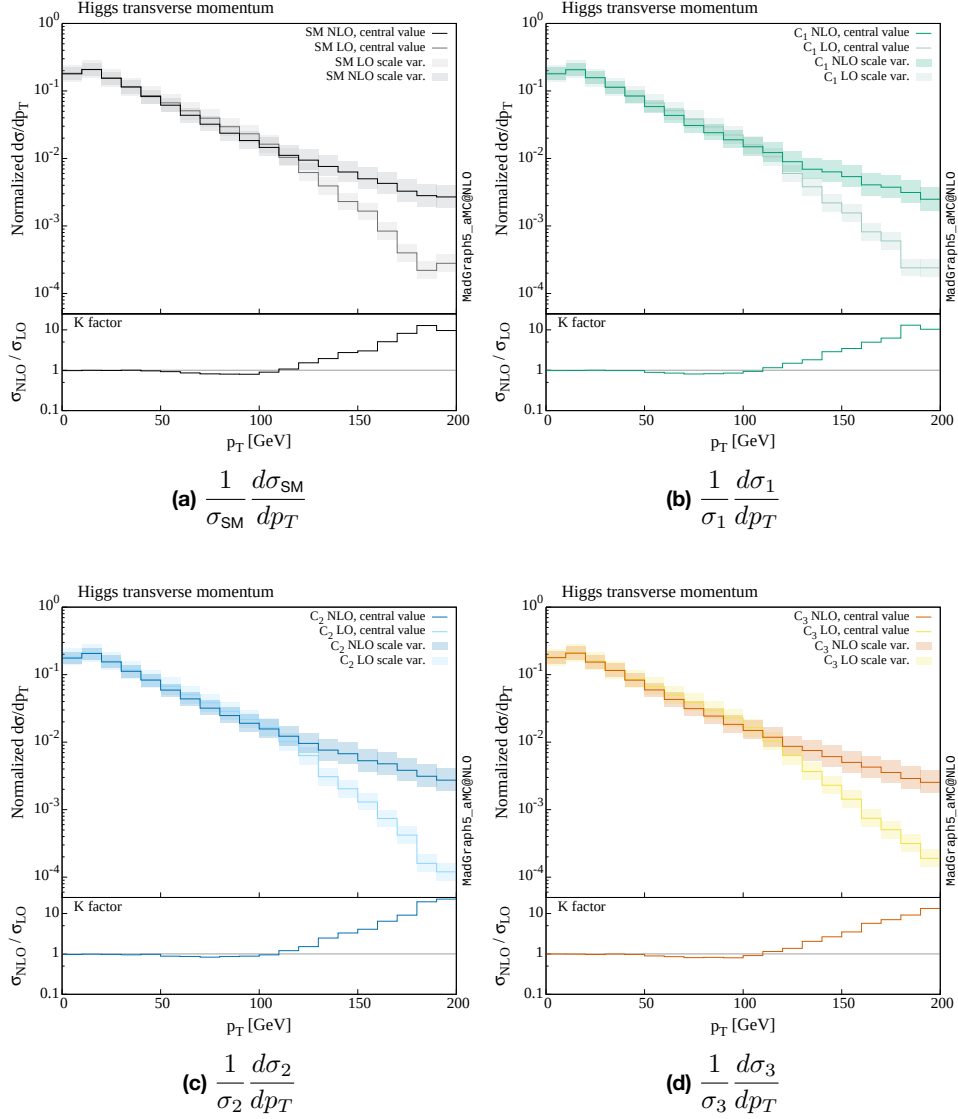
Figure 6.3: Comparison of the LO and NLO shapes of the transverse momentum spectra of \sigma_{\text{SM}} and the \sigma_i . The inserts show the ratios of the differential cross sections at LO and at NLO.
