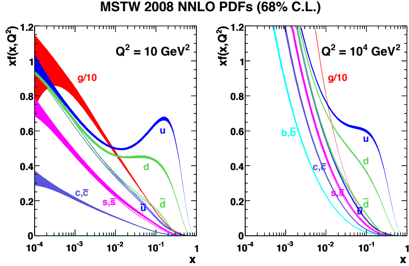
Figure 2.6: Examples of PDF from the MSTW2008 fit [77].
