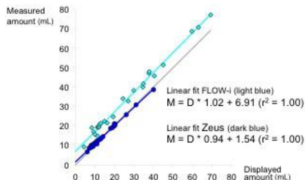
[Fig. 1. Displayed (D) versus measured (M) amount of desflurane (in mL of liquid) with each of the machines. Straight line = linear fit. Color code of line and data points: light blue = FLOW-i, dark blue = Zeus. Gray = line of identity]
