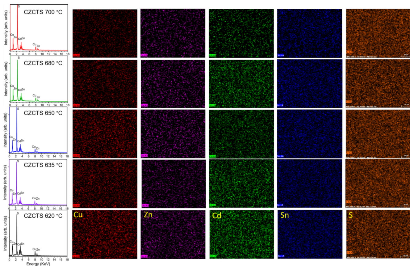
FIGURE 4 | EDS spectra, and the surface EDS mapping of the components elements of the sample sulfurized at different temperature. [Color figure can be viewed at wileyonlinelibrary.com ]
