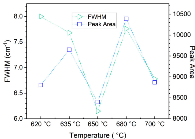
FIGURE 3 | FWHM and peak area of A 335 /B (LO) 335 vibration mode of the CZCTS samples. [Color figure can be viewed at wileyonlinelibrary.com ]
