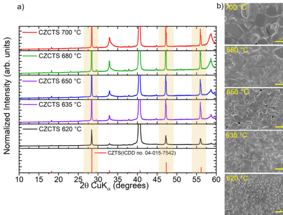
FIGURE 1 | (a) XRD and (b) SEM images of CZCTS thin films sulfurized at different temperature. All bars correspond to 1 \mu\text{m} (Mag = 10.00 KX). [Color figure can be viewed at wileyonlinelibrary.com ]
