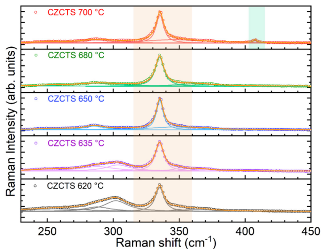
FIGURE 2 | Raman spectroscopy of CZCTS thin films. [Color figure can be viewed at wileyonlinelibrary.com ]
