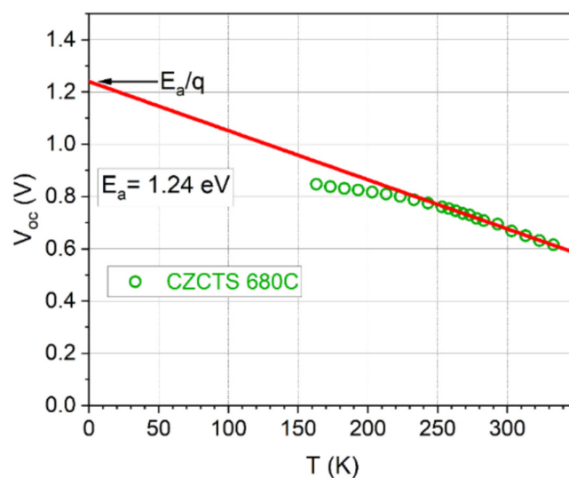
FIGURE 7 | Temperature dependence and linear extrapolation of V_{oc} . The 0 K intercept of the extrapolation is defined as activation energy E_a . [Color figure can be viewed at wileyonlinelibrary.com ]
