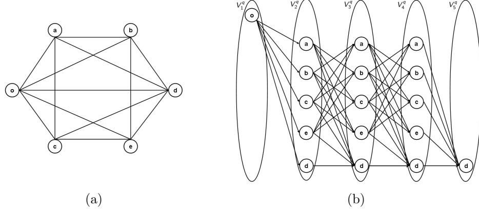
Figure 1: Original network (a) and its alternative (or associated) layered representation (b) when L = 4
