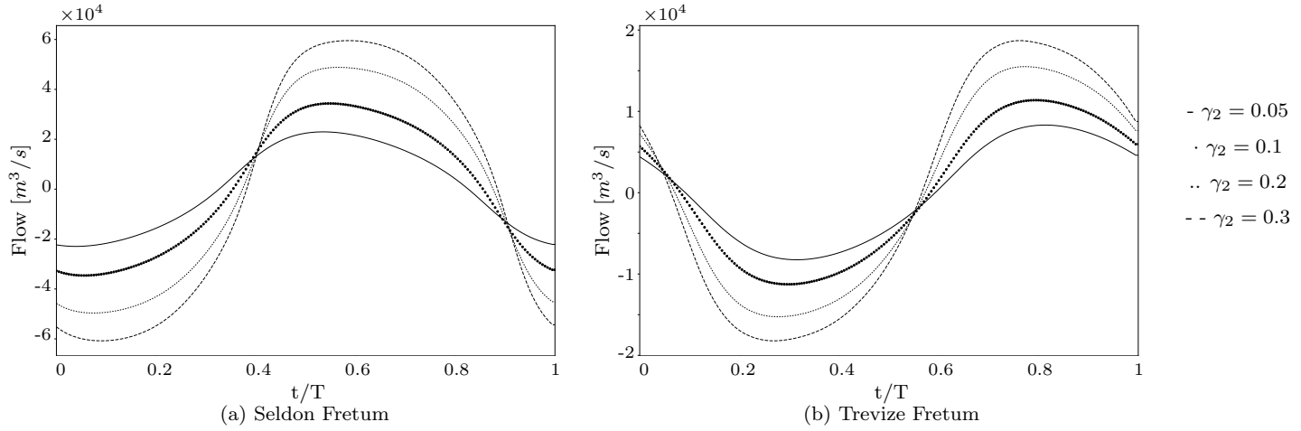
Figure 13: Volumetric flow rate through Seldon (a) and Trevize Fretum (b) over one Titan day for \gamma_2 ranging from 0.05 to 0.3. In Seldon and Trevize Fretum, it is respectively positive towards Kraken 1 and Ligeia Mare. In each strait, the volumetric flow rate increases with \gamma_2 and a small time lag appears.
