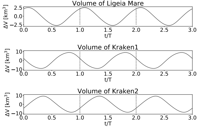
Figure 8: Volume variation in the basins of Kraken and Ligeia Maria over three Titan days. The variation is larger in both basins of Kraken Mare than in Ligeia Mare and the total variation of each basin over a Titan day is nil.
