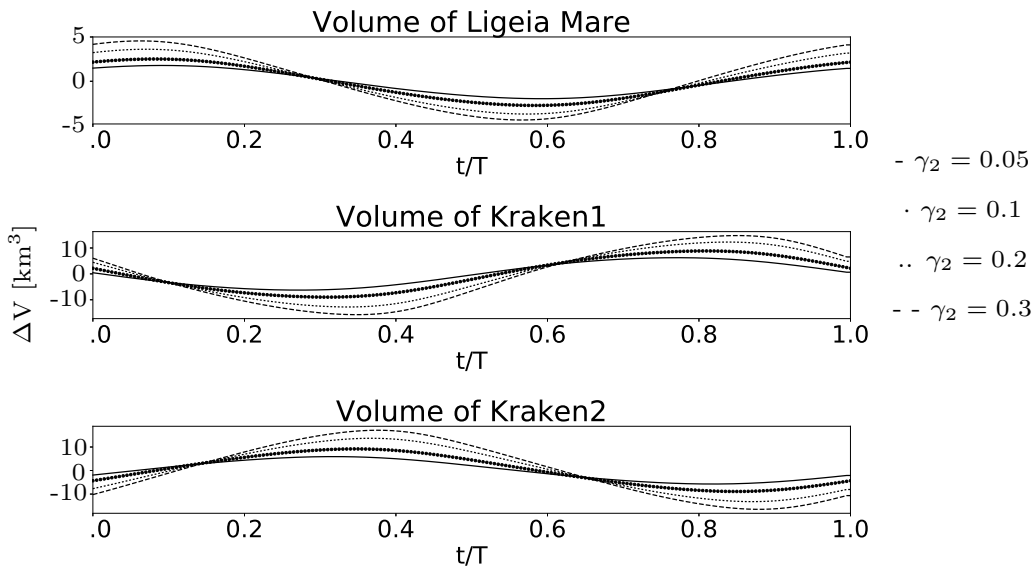
Figure 14: Variation of volume in both basins of Kraken Mare and Ligeia Mare over one Titan day. In each basin, a time lag appears and the maximum volume variation rises when \gamma_2 increases.
