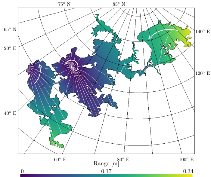
(a) H = 20\text{ m}
