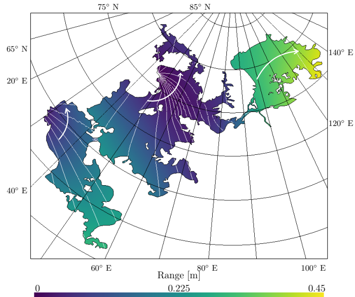
(b) H = 50\text{ m}
