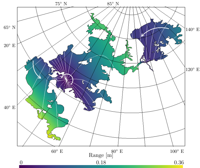
(a) Tidal range and phase for bathy A
