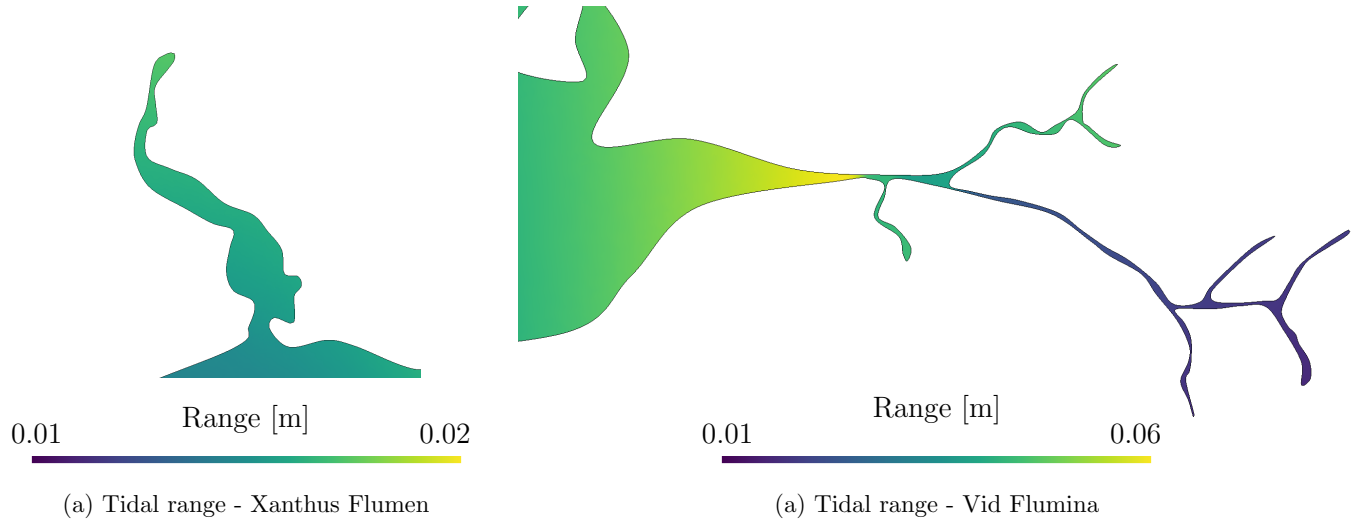
Figure 10: Tidal range in canyons near Xanthus flumen (a) and near Vid Flumina (b) for the reference case. The areas shown in these figures correspond to red rectangles D and C in Fig.1.
