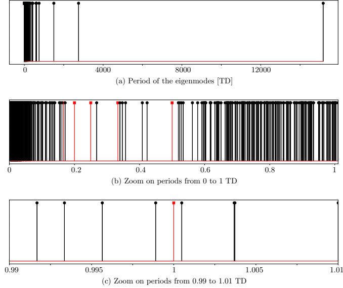
Figure 6: Periods of the northern seas eigenmodes (Panel (a), in TD ) with a zoom from 0 to 1 TD (Panel (b)) and from 0.99 to 1.01 TD (Panel (c)). The tidal period and its first fifth integer divisors are in red.
