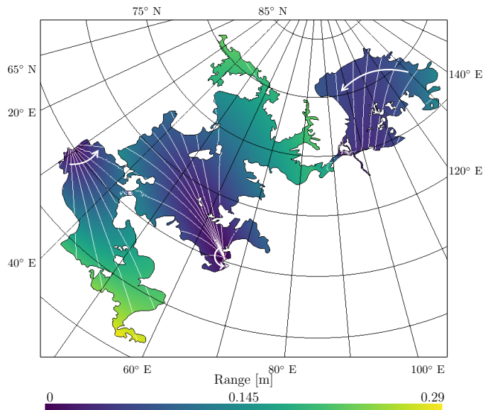
Figure 2: Tidal range (in m ) and tidal phase (white lines, with a 15^\circ spacing) of the first tidal component (whose period is 1 TD ) in Kraken and Ligeia Maria. The white arrows show the direction of the tide. The tidal range is the surface elevation difference between high tide and low tide. There is an amphidromic point in Kraken 1 (at 65.213^\circ N , 66.459^\circ E ) but not in Kraken 2 or Ligeia Mare. The tidal phase at each end of the Seldon and Trevize Fretum are not the same, which results in strong transition in the straits. This is also observed for the tidal range. Such phenomenon suggests independent tidal motion in each basin. The tidal range is maximum in the south-eastern part of Kraken 2.
