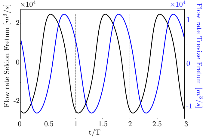
Figure 7: Volumetric flow rate through Seldon (black line) and Trevize Fretum (blue line) over three Titan days. In Seldon and Trevize Fretum, it is respectively positive towards Kraken 1 and Ligeia Mare. The volumetric flow rate through the former is about three times larger than that through the latter. The net difference over 1 TD is 0 \text{ km}^3 .
