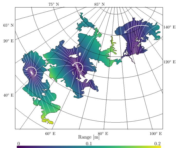
(b) Tidal range and phase for bathy B
