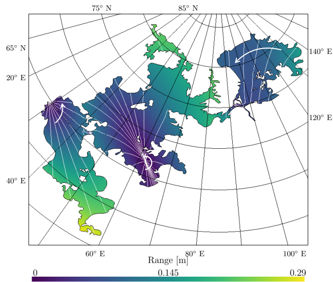
Figure 15: Tidal range (in m ) and tidal phase (white lines, with a 15^\circ spacing) in Kraken and Ligeia Maria for H = 10 m . The white arrows show the direction of the tide. The tide rotates anticlockwise and the amphidromic point in Kraken 1 moved with respect to its location for the reference case. The location and value of the maximum tidal range do not change significantly with respect to the reference case.
