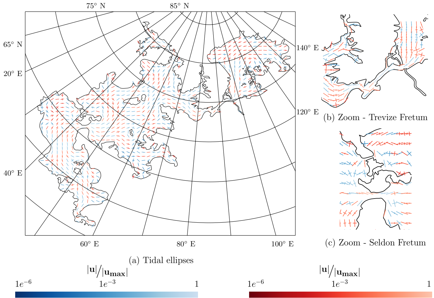
Figure 5: Major and minor axes of the tidal ellipses in the northern seas (Panel (a)), Trevize Fretum (Panel (b)) and Seldon Fretum (Panel (c)). The tidal ellipses represent the orientation of the first tidal component current over a whole period. Red and blue ellipses respectively indicate an anti-clockwise/clockwise rotation while the color scales with the magnitude of the maximum velocity over 1 TD . The smaller the minor axis, the more elongated the ellipses and the more unidirectional the velocity.
