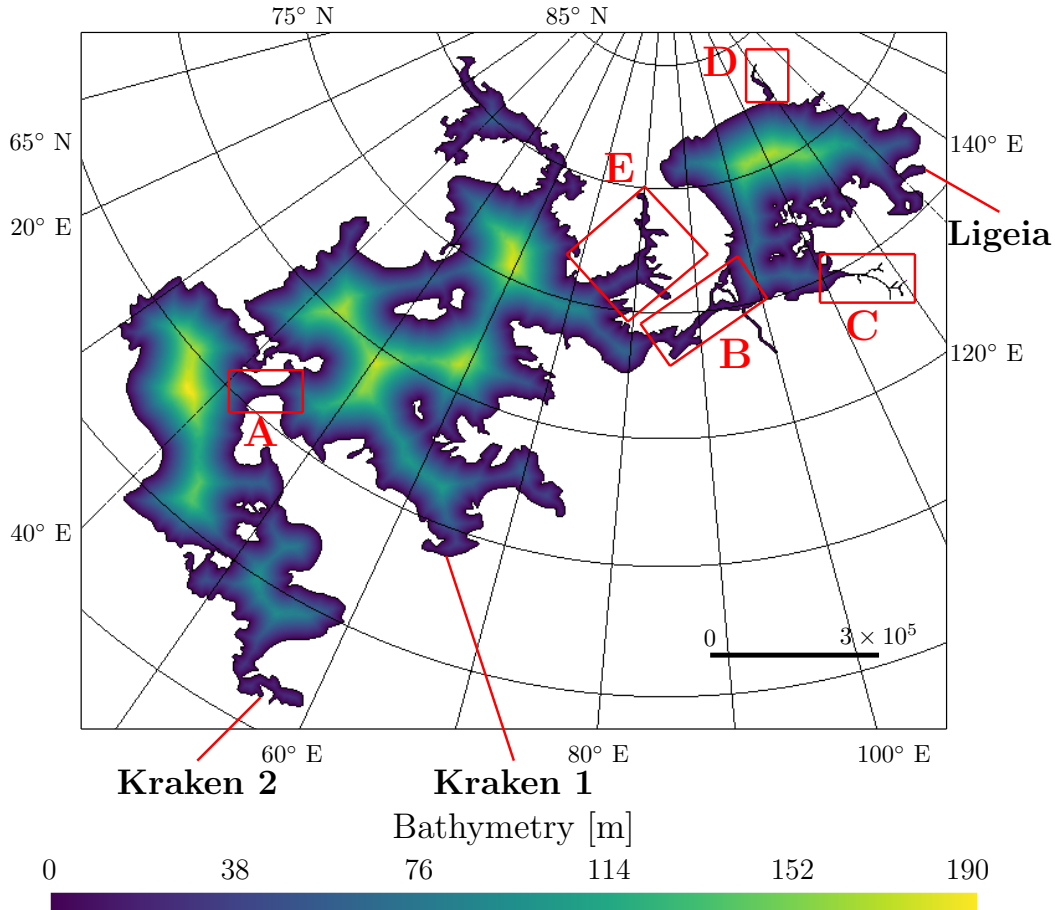
Figure 1: Bathymetry map of Kraken and Ligeia Maria. The depth scales with the distance to the nearest shore, similarly to the bathymetry of Lorenz et al. (2014). The red letters refer respectively Seldon Fretum (A), Trevize Fretum (B), the canyons next to Vid flumina (C) and Xanthus Flumen (D), and Moray Sinus (E).
