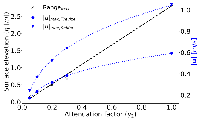
Figure 11: Maximal tidal range (cross, in m ) and maximum fluid speed in Trevize (circle, in m/s ) and Seldon (triangle, in m/s ) Fretum as function of the attenuation factor \gamma_2 . The dashed and dotted lines are respectively a linear and a quadratic mean square root approximation.
