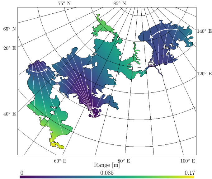
(a) Tidal range and phase for \gamma_2 = 0.05
