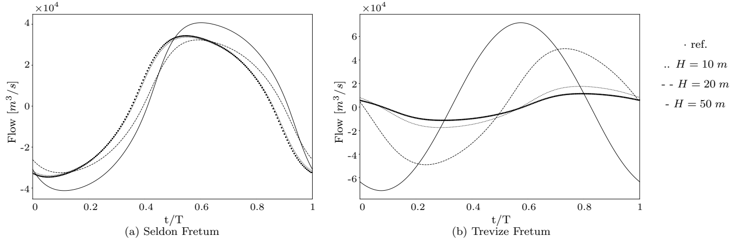
Figure 17: Volumetric flow rate through Seldon (a) and Trevize Fretum (b) over one Titan day for the reference case and the three depths implemented. In Seldon and Trevize Fretum, it is respectively positive towards Kraken 1 and Ligeia Mare. The volumetric flow rate in Seldon Fretum is less sensitive to this parameter than that in Trevize but it still increases and is lagged when H varies. The volumetric flow rate in Trevize Fretum increases with H and a time lag appears.
