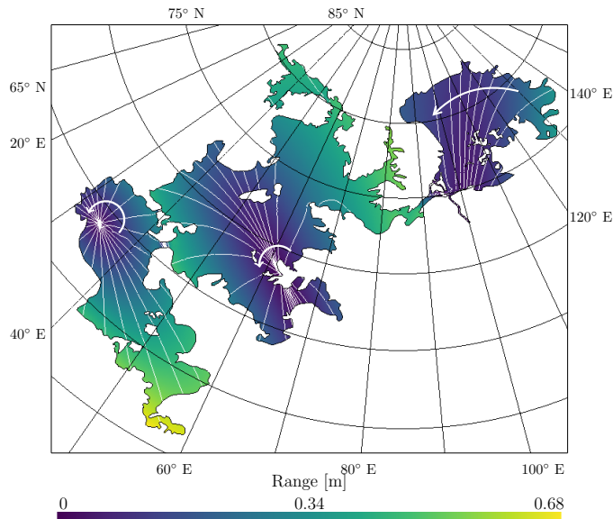
(b) Tidal range and phase for \gamma_2 = 0.3
