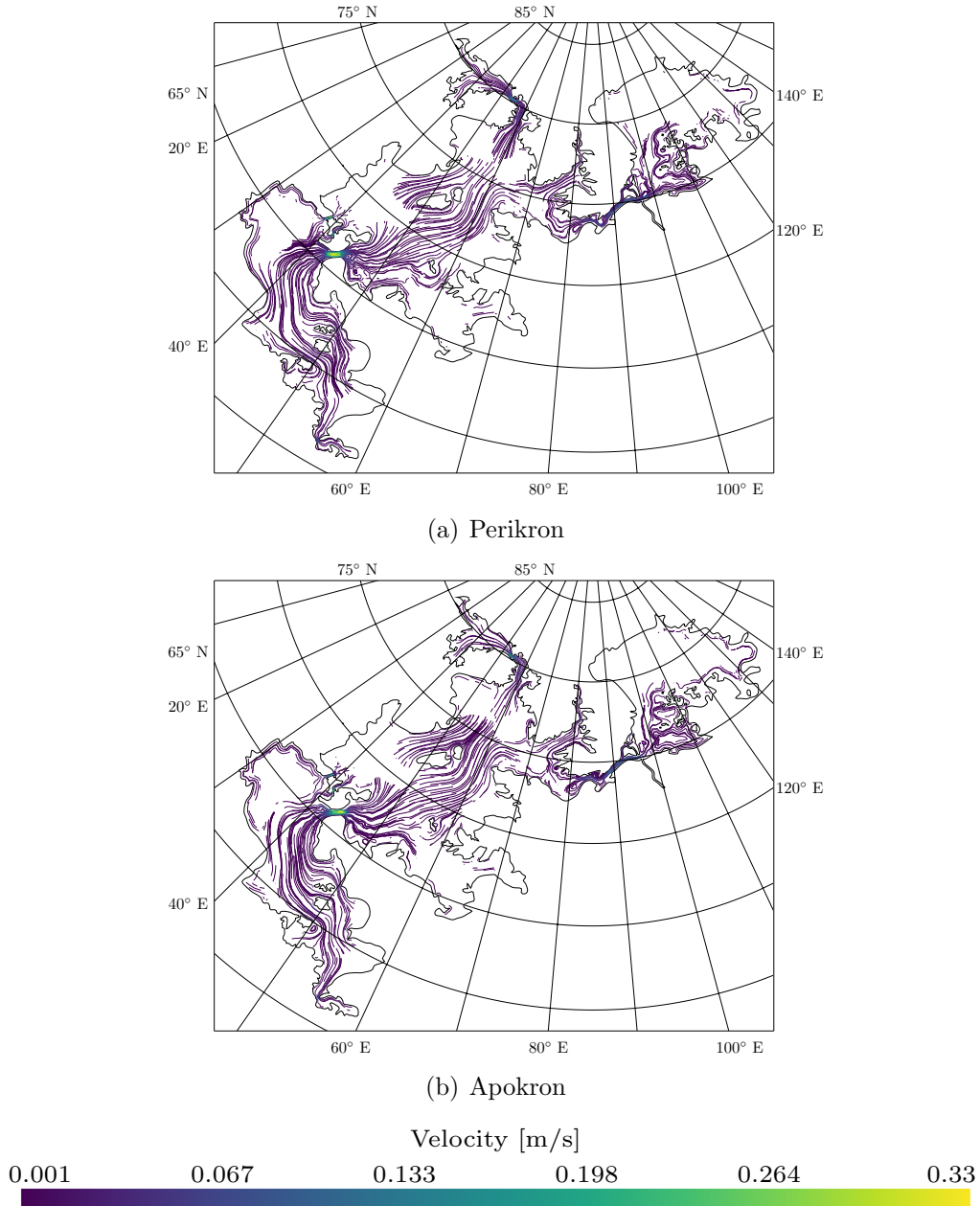
Figure 3: Tidal current streamlines at Perikron (a) and Apokron (b). The empty areas correspond to areas where the predicted velocity field magnitude is smaller than 0.001 \text{ m/s} . At these periods, the main current pattern is a flux going from the south-eastern part of Kraken 2 towards the north of Kraken 1 and from Moray Sinus towards Ligeia Mare (Panel (b)) or in the opposite direction (Panel (a)).
