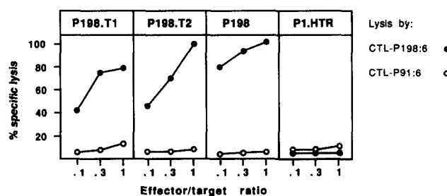
Figure 3. Lysis of P1.HTR genomic transfectants (P198.T1 and T2) and of control targets by anti-P198 CTL clone CTL-P198:6 in a 4-h ^{51}\text{Cr} release assay. Lysis by CTL-P91:6, which is directed against unrelated \text{tum}^- antigen P91A, is also shown.
