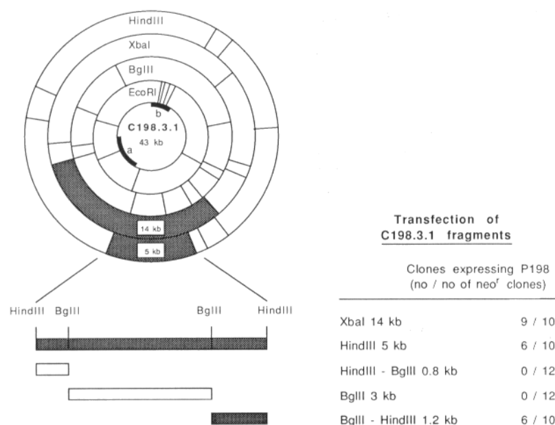
Figure 4. Restriction map of C198.3.1 and identification of fragments transferring the expression of antigen P198. Restriction fragments of C198.3.1, which were all cloned in pUC vectors with the exception of the 14-kb XbaI fragment, were cotransfected into P1.HTR with pSVtkneo \beta . The drug-resistant cells were selected, and clones were tested for lysis by CTL-P198:6 in a visual assay. Regions containing sequences of the cosmid vector are marked a and b . Subsequent analysis revealed that in this cosmid, gene P198 is interrupted at position 4176 (see Figs. 5 and 6), immediately before the HindIII site of the cosmid, which is located at the end of the 1.2-kb BglII-HindIII fragment.
