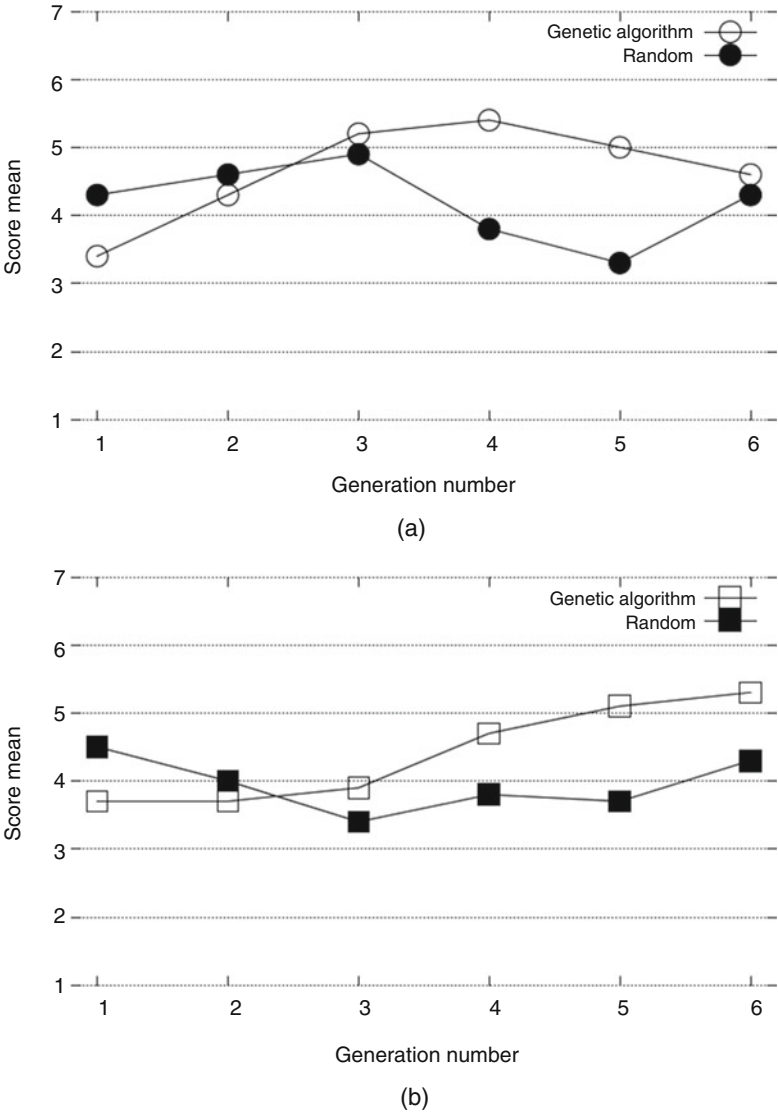
Fig. 3.10 Comparing variant selection based on genetic algorithm and random. (a) LIST. (b) SnT
