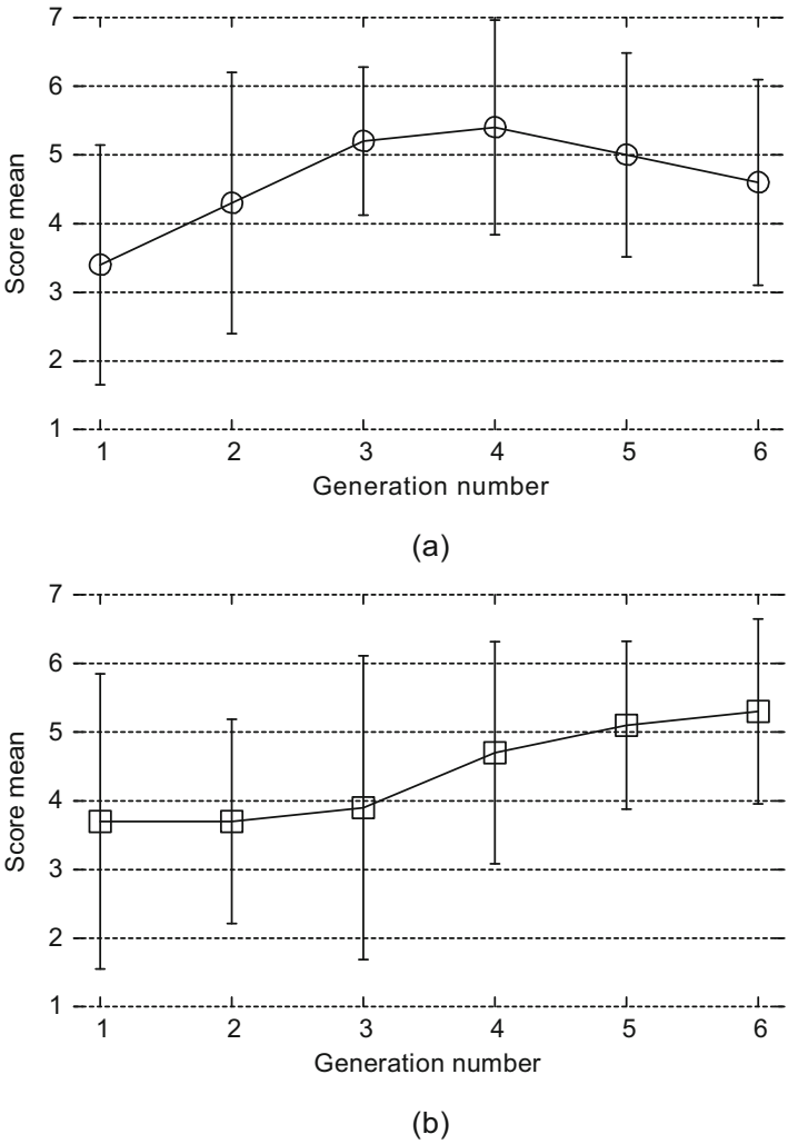
Fig. 3.8 Results of the genetic algorithm evolution in the two organizations. (a) LIST. (b) SnT
