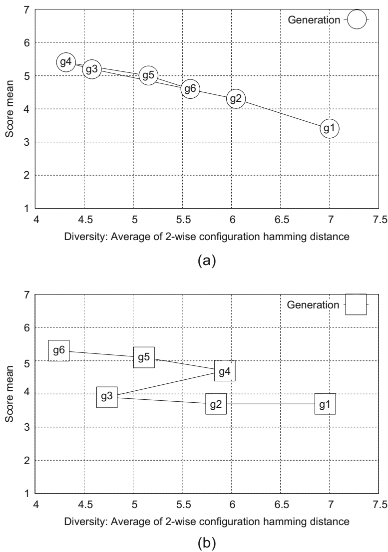
Fig. 3.9 Generations progress in terms of mean score and diversity. (a) LIST. (b) SnT
