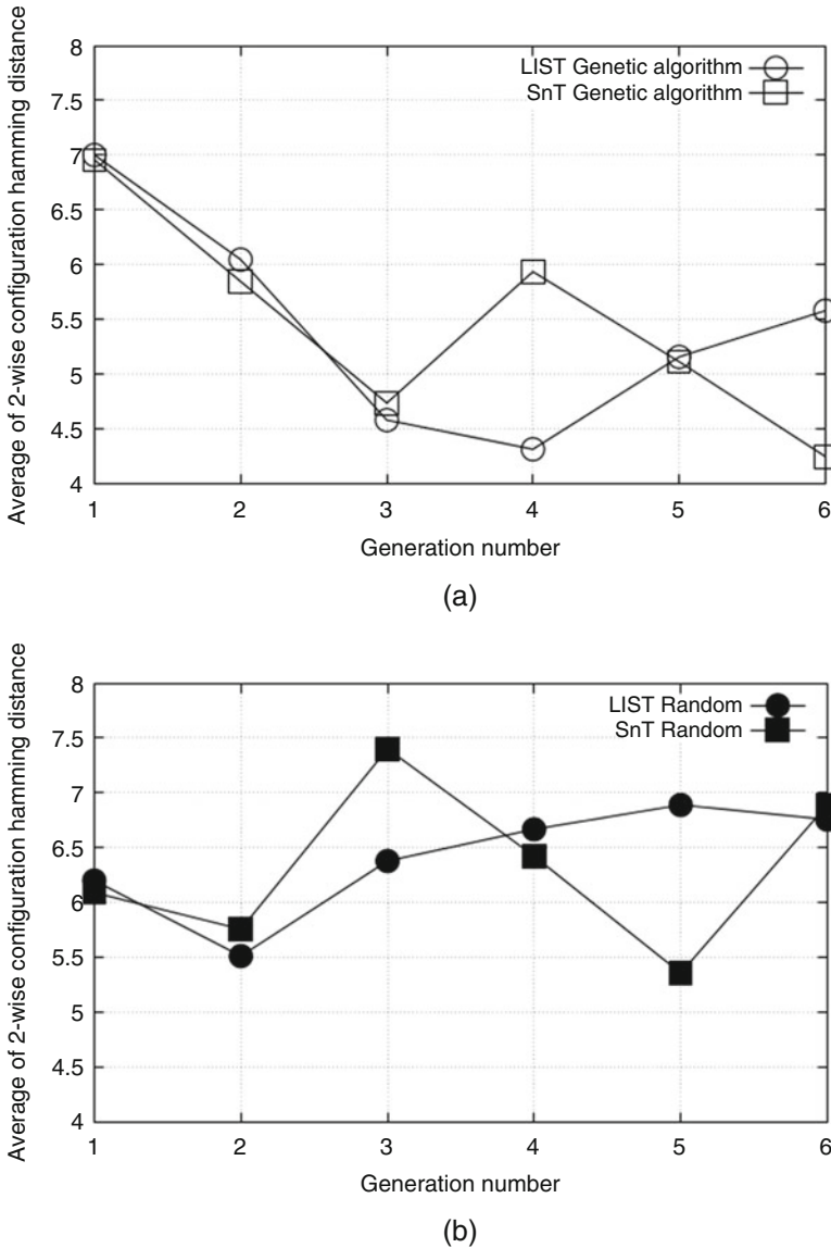
Fig. 3.11 Genotype population diversity. (a) Genetic algorithm. (b) Random
