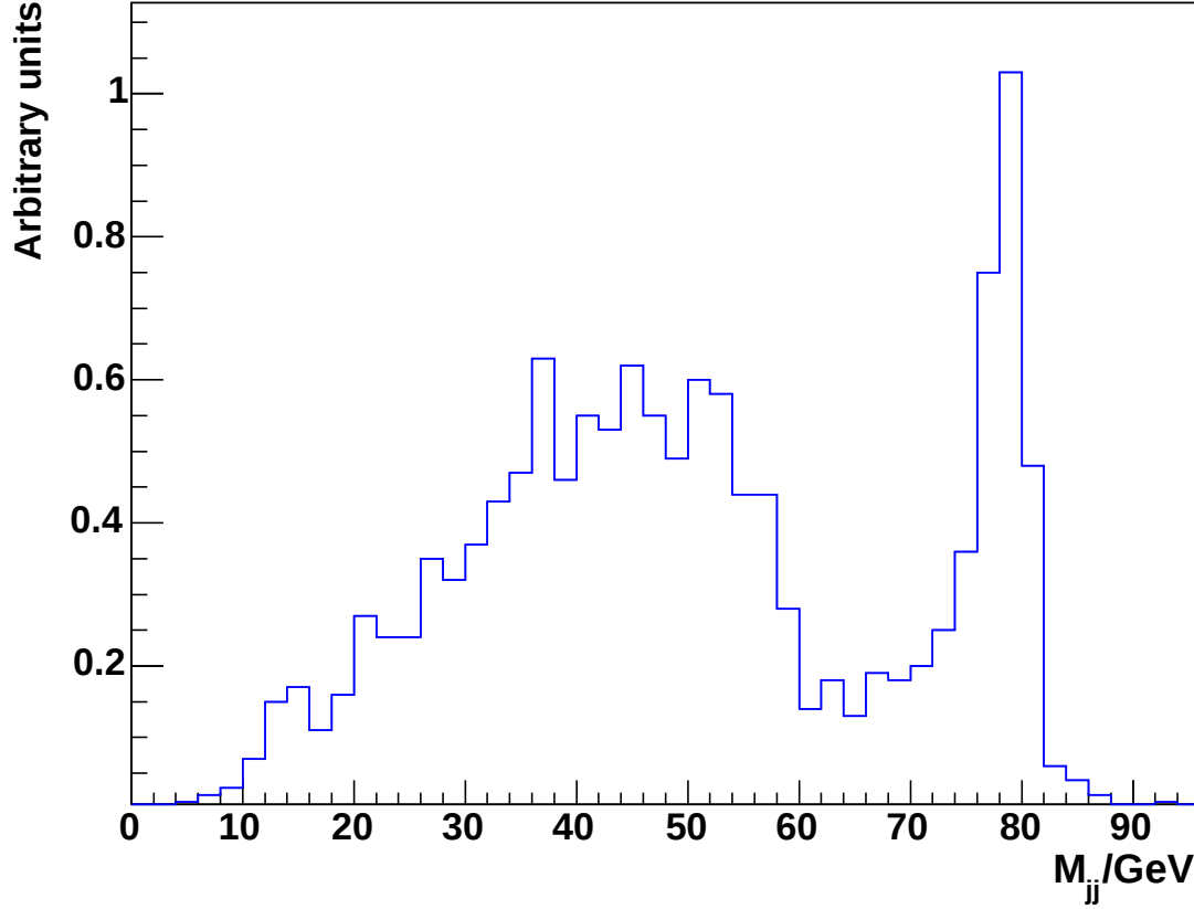
Fig. 6: The di-jet invariant mass distribution dN/dM_{jj} in the semi-leptonic decay channel H \rightarrow WW^* \rightarrow l\nu jj for M_H = 140 GeV.
