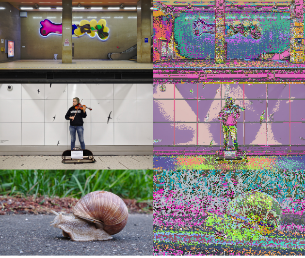
Figure 3. Segmentation of three test images [1]: each distinct color represents one of 64 CDF tables used to encode a latent spatial location ( 16 \times 16 pixels patch)
