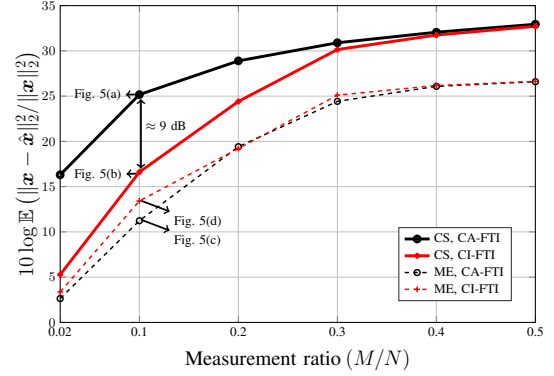
Fig. 4: Reconstruction performance of Minimum Energy (ME) ( i.e. , applying the pseudo-inverse of \Phi_\Omega ) and Compressive Sensing (CS) frameworks for CA-FTI and CI-FTI. The results are averaged over 10 trials ( i.e. , over the random selection of \Omega ). Noise level is set such that 10 \log (\|\Phi_\Omega \mathbf{x}\|_2^2 / \|\mathbf{n}\|_2^2) = 10 dB. As explained in the text (and also by the \ell_2 - \ell_1 instance optimality of (2) [5]) CA-FTI needs less number of samples than CI-FTI. Moreover, regardless of measurement ratio ME solution results in poor quality images.
