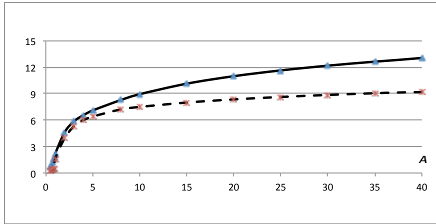
Figure 1: Optimal output \bar{Y} (in logarithmic scale) for various values of the economic efficiency A in two cases: no deterioration, \delta = 0 (a solid line) and with deterioration (a dashed line) at \delta = 0.01 .
