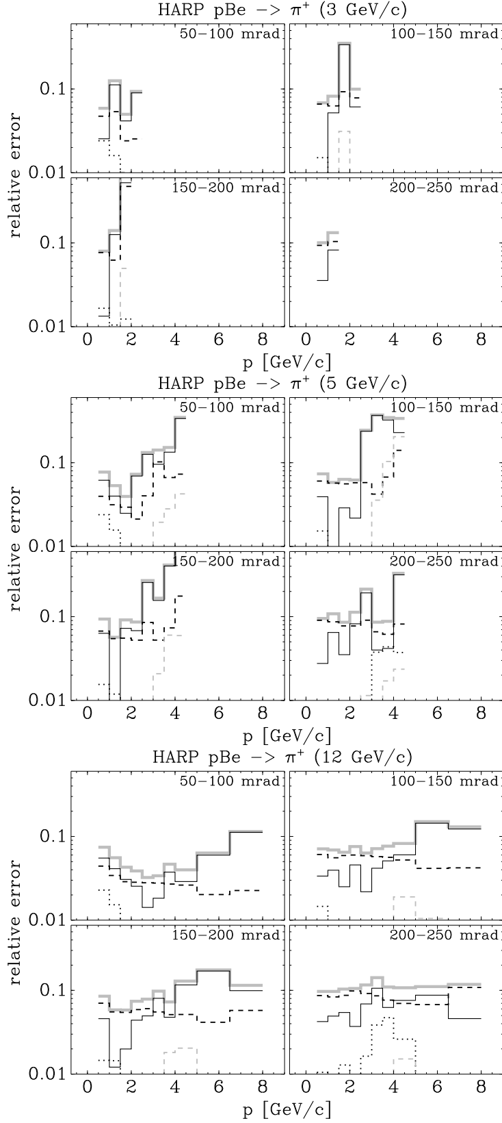
FIG. 2: Total systematic error (grey solid line) and main components: black short-dashed line for absorption+tertiaries interactions, black dotted line for track efficiency and target pointing efficiency (mostly \leq 1\% ), black solid line for momentum scale+resolution and angle scale for a typical target (Be) at some typical incident momenta.
