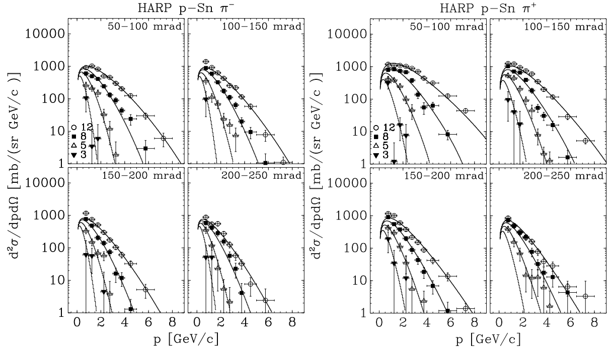
FIG. 7: p-Sn differential cross sections: left panel \pi^- production, right panel \pi^+ production. The curves represent the global parametrization as described in the text. In the top right corner of each plot the covered angular range is shown in mrad.
