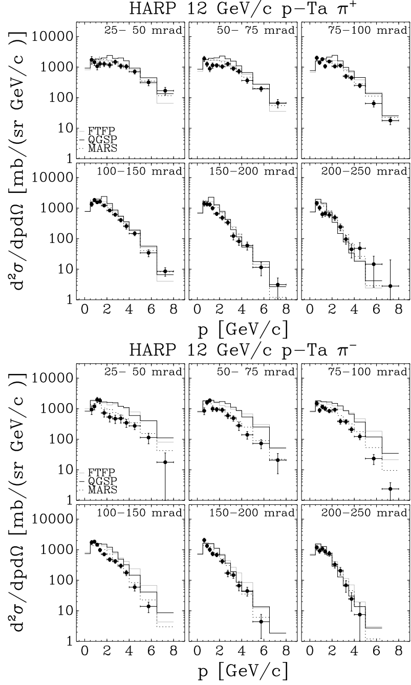
FIG. 20: Comparison of HARP double-differential \pi^\pm cross sections for p-Ta at 12 GeV/c with GEANT4 and MARS MC predictions, using several generator models (see text for details): FTFP model dotted grey line, QGSP model black solid line, MARS dashed line.
