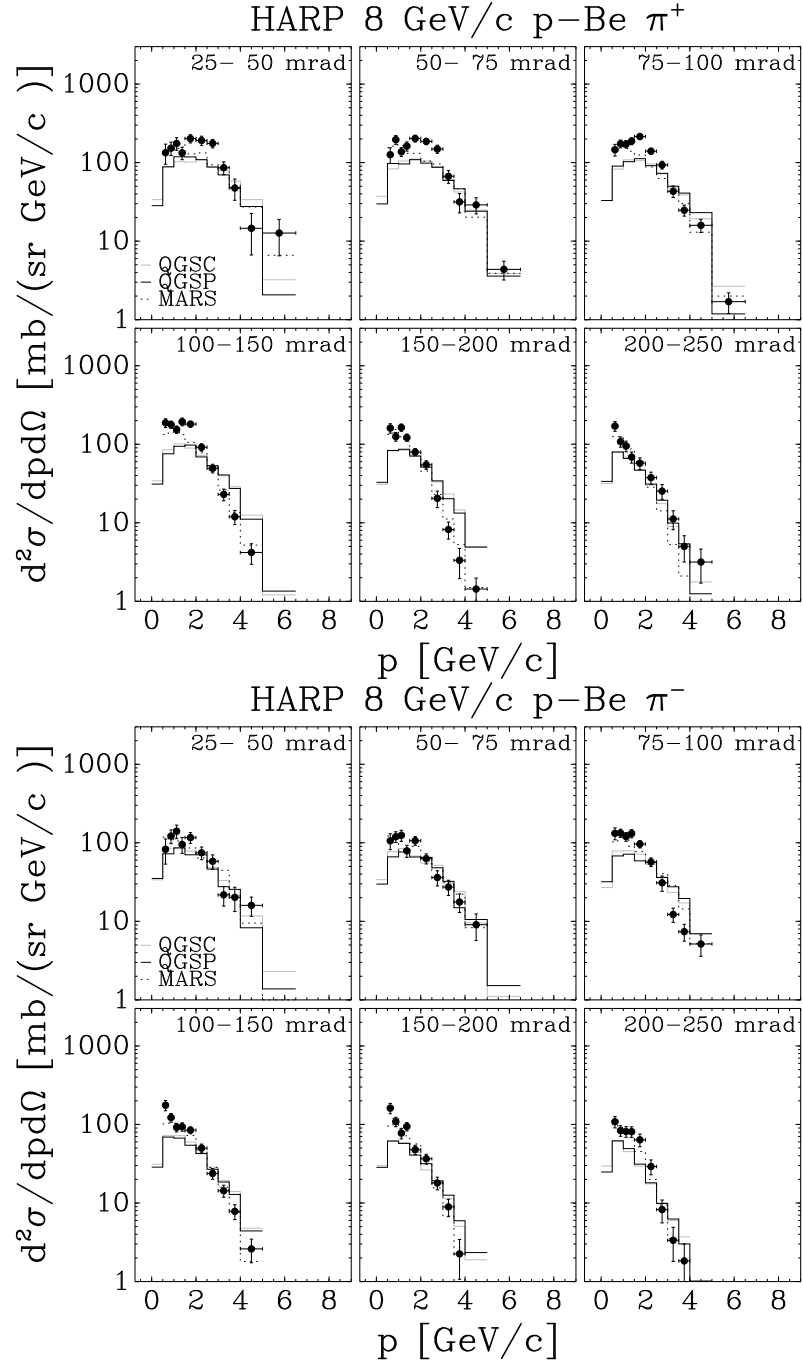
FIG. 15: Comparison of HARP double-differential \pi^\pm cross sections for p-Be at 8 GeV/c with GEANT4 and MARS MC predictions, using several generator models (see text for details): QGSC model dotted line, QGSP model black solid line, MARS model dashed line.
