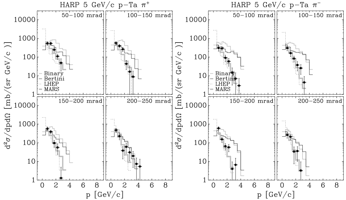
FIG. 18: Comparison of HARP double-differential \pi^\pm cross sections for p-Ta at 5 GeV/c with GEANT4 and MARS MC predictions, using several generator models (see text for details): Binary model grey line, Bertini model black solid line, LHEP model dotted line, MARS model grey solid line.
