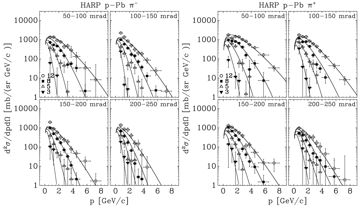
FIG. 9: p-Pb differential cross sections: left panel \pi^- production, right panel \pi^+ production. The curves represent the global parametrization as described in the text. In the top right corner of each plot the covered angular range is shown in mrad.
