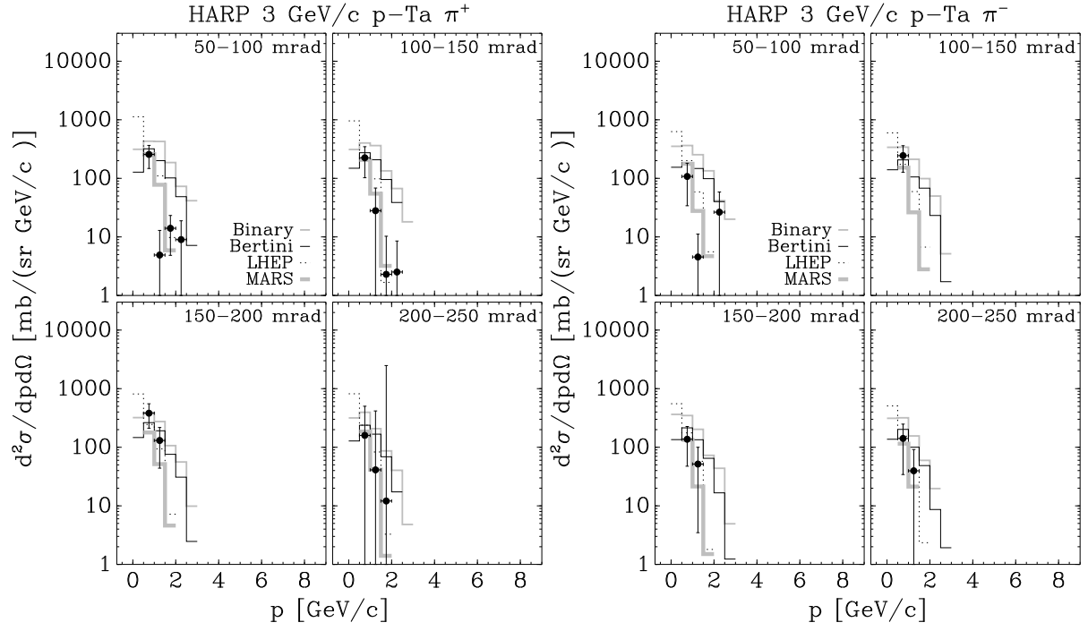
FIG. 17: Comparison of HARP double-differential \pi^\pm cross sections for p-Ta at 3 GeV/c with GEANT4 and MARS MC predictions, using several generator models (see text for details): Binary model grey line, Bertini model black solid line, LHEP model dotted line, MARS model grey solid line.
