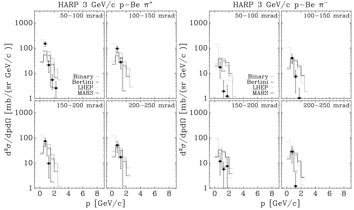
FIG. 13: Comparison of HARP double-differential \pi^\pm cross sections for p-Be at 3 GeV/c with GEANT4 and MARS MC predictions, using several generator models (see text for details): binary model grey line, Bertini model black solid line, LHEP model dotted line, MARS model grey solid line.
