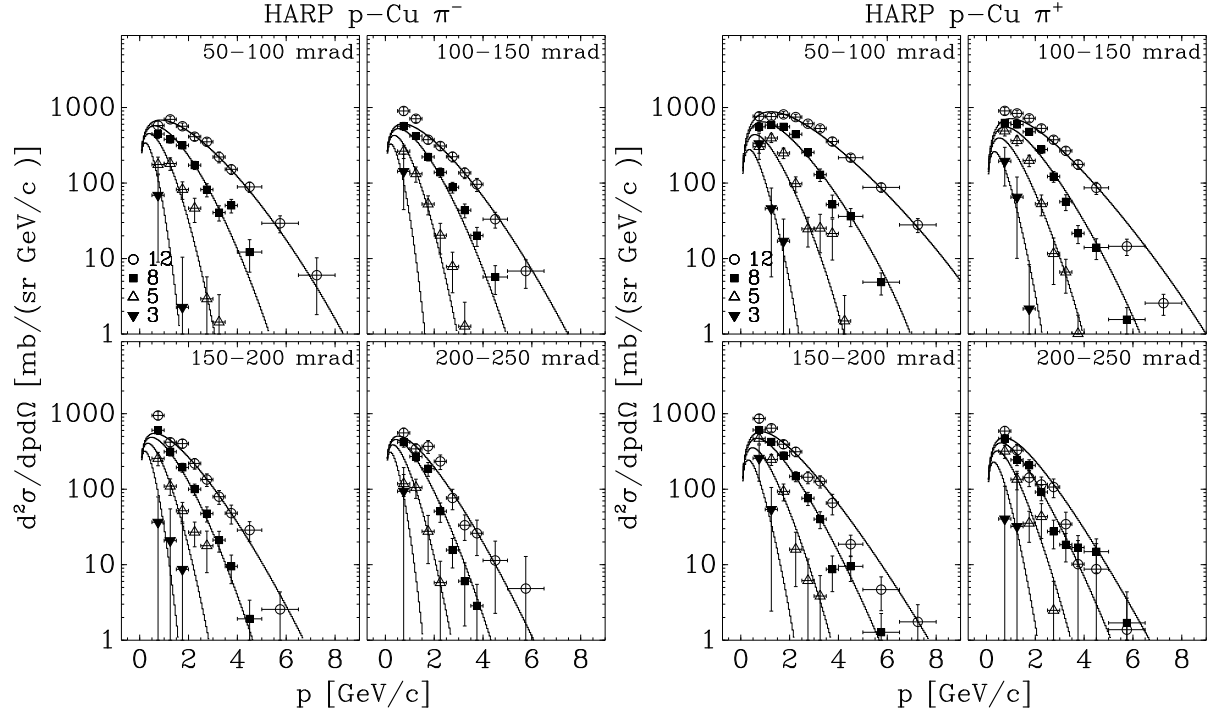
FIG. 6: p-Cu differential cross sections: left panel \pi^- production, right panel \pi^+ production. The curves represent the global parametrization as described in the text. In the top right corner of each plot the covered angular range is shown in mrad.
