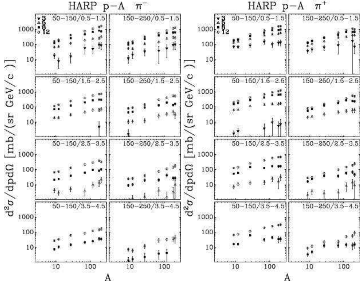
FIG. 11: The dependence on the atomic number A of the pion production yields in p -Be, p -Al, p -C, p -Cu, p -Sn, p -Ta, p -Pb interactions averaged over two forward angular regions ( 0.05 \text{ rad} \leq \theta < 0.15 \text{ rad} and 0.15 \text{ rad} \leq \theta < 0.25 \text{ rad} ) and four momentum regions ( 0.5 \text{ GeV}/c \leq p < 1.5 \text{ GeV}/c , 1.5 \text{ GeV}/c \leq p < 2.5 \text{ GeV}/c , 2.5 \text{ GeV}/c \leq p < 3.5 \text{ GeV}/c and 3.5 \text{ GeV}/c \leq p < 4.5 \text{ GeV}/c ), for the four different incoming beam energies.
