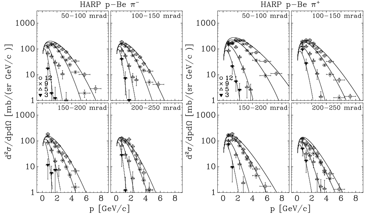
FIG. 3: p-Be differential cross sections: left panel \pi^- production, right panel \pi^+ production. The curves represent the global parametrization as described in the text. In the top right corner of each plot the covered angular range is shown in mrad.
