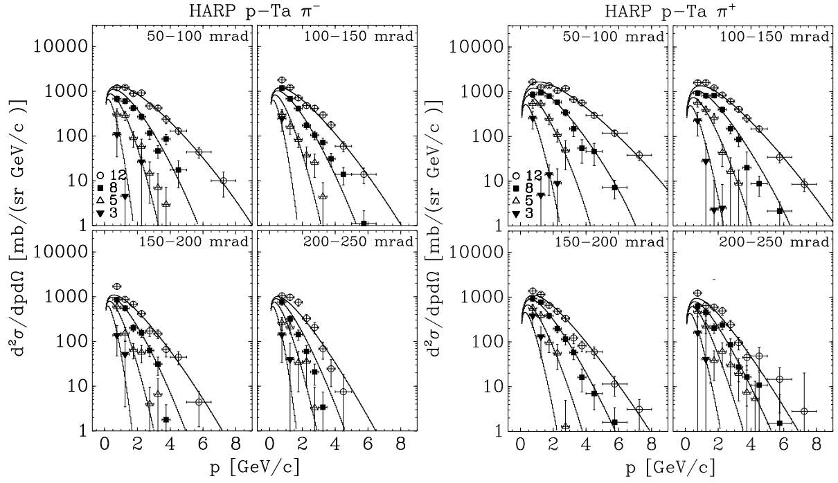
FIG. 8: p-Ta differential cross sections: left panel \pi^- production, right panel \pi^+ production. The curves represent the global parametrization as described in the text. In the top right corner of each plot the covered angular range is shown in mrad.
