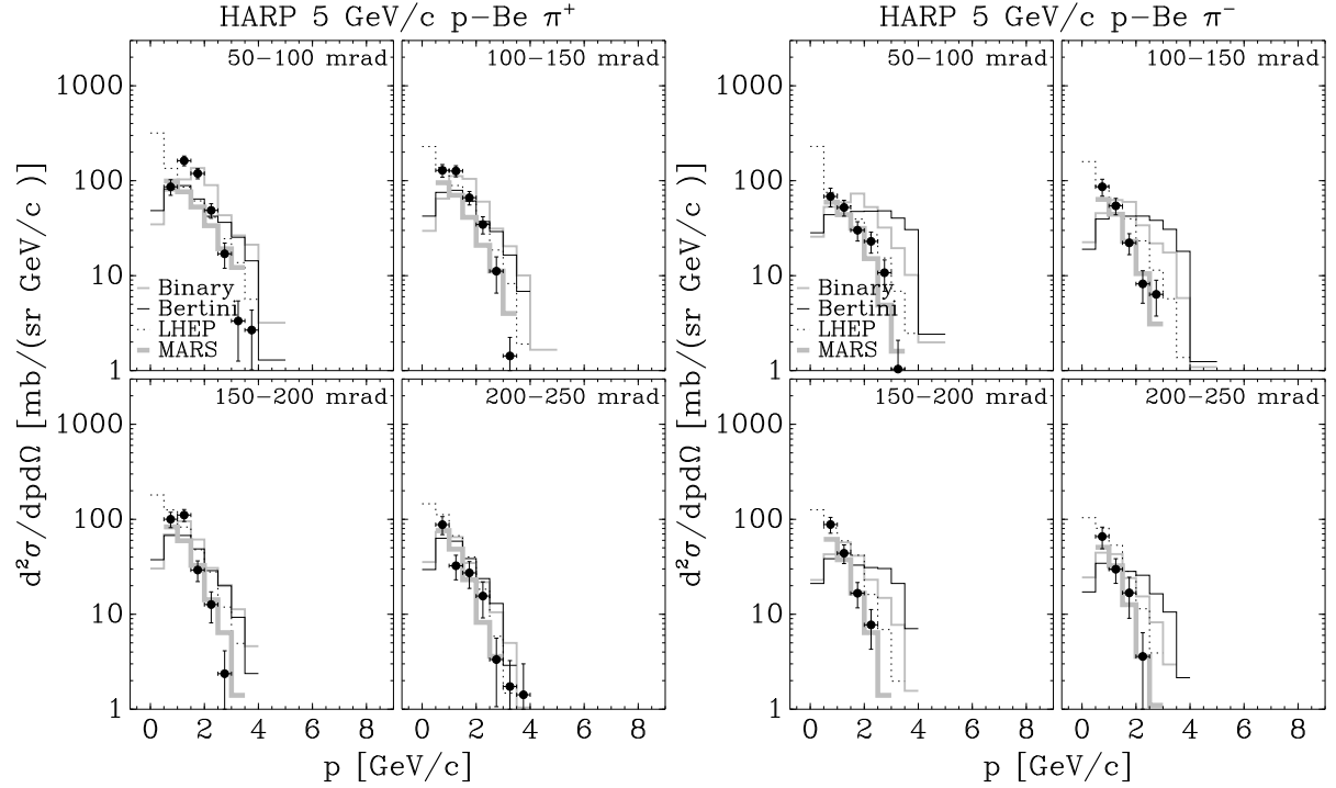
FIG. 14: Comparison of HARP double-differential \pi^\pm cross sections for p-Be at 5 GeV/c with GEANT4 and MARS MC predictions, using several generator models (see text for details): Binary model grey line, Bertini model black solid line, LHEP model dotted line, MARS model grey solid line.
