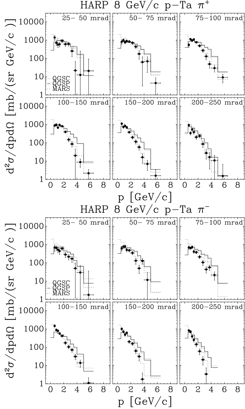
FIG. 19: Comparison of HARP double-differential \pi^\pm cross sections for p-Ta at 8 GeV/c with GEANT4 and MARS MC predictions, using several generator models (see text for details): QGSC model dotted line, QGSP model black solid line, MARS dashed line.
