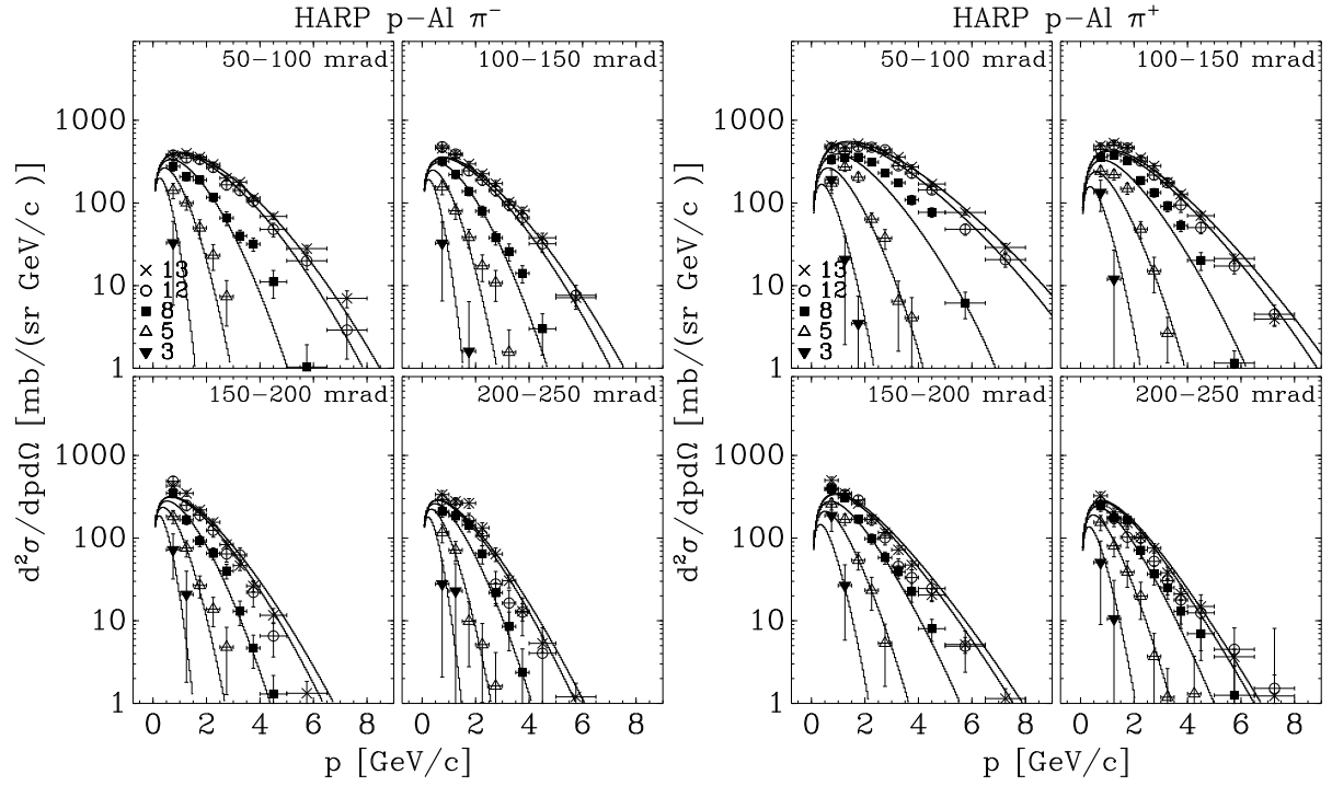
FIG. 5: p-Al differential cross sections: left panel \pi^- production, right panel \pi^+ production. The curves represent the global parametrization as described in the text. In the top right corner of each plot the covered angular range is shown in mrad.
