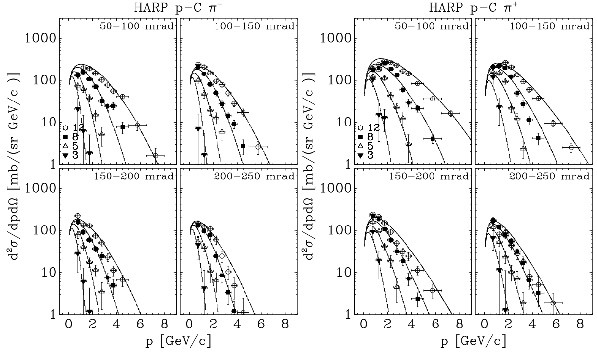
FIG. 4: p-C differential cross sections: left panel \pi^- production, right panel \pi^+ production. The curves represent the global parametrization as described in the text. In the top right corner of each plot the covered angular range is shown in mrad.
