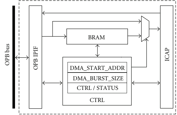
FIGURE 1: Reconfiguration controller.
