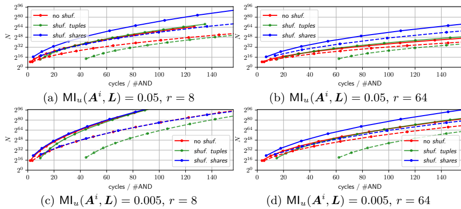
Figure 10: Cycles vs. security for 512 bitwise ANDs for various noise levels and randomness cost. Continuous are for bs = 32 and dashed ones for bs = 16 . The leftmost bullets stand for d = 2 and the value of d is increased by one for each step of the curves.
