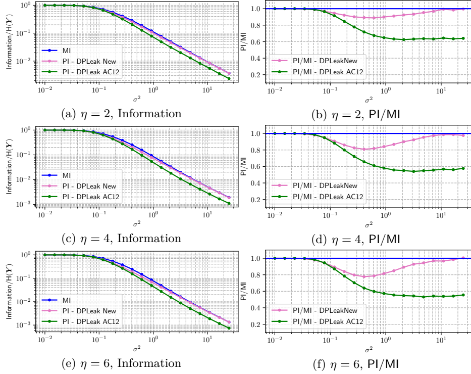
Figure 1: IT analysis of shuffled implementation Algorithm 2 . Normalized IT metrics are on the left. The ratios between the PIs and the MI are on the right.
