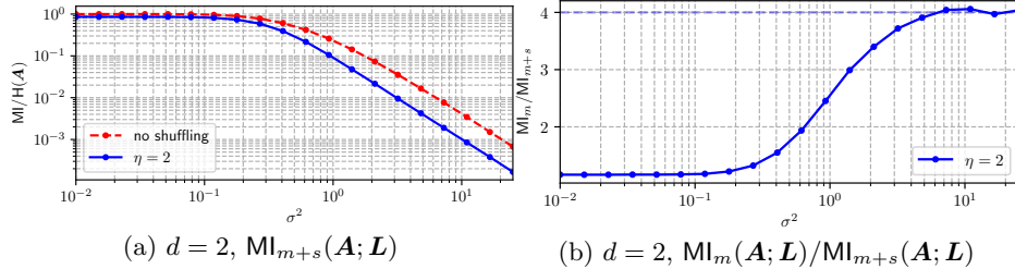
Figure 7: Shuffling ISW shares ( Algorithm 7 , config. (0^i, 0^j, 1^s) ): IT analysis.
