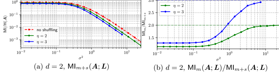
Figure 6: Shuffling ISW multiplication tuples (Algorithm 6): IT analysis.
