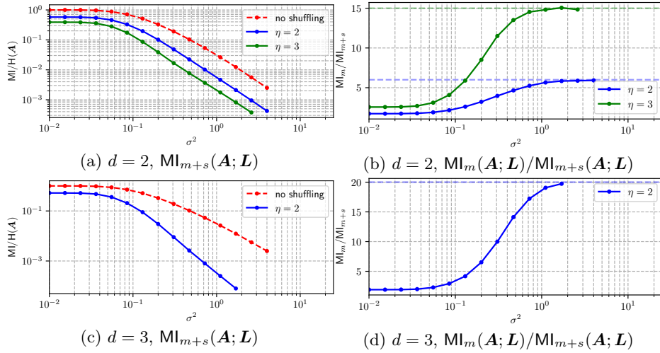
Figure 5: Shuffling everything ( Algorithm 5 ): IT analysis.
