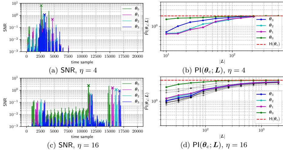
Figure 12: IT analysis of real permutation leakages. Left: SNR in function of the time. Right: Information on permutation indexes \theta_i versus dimension of the leakage |L| .
