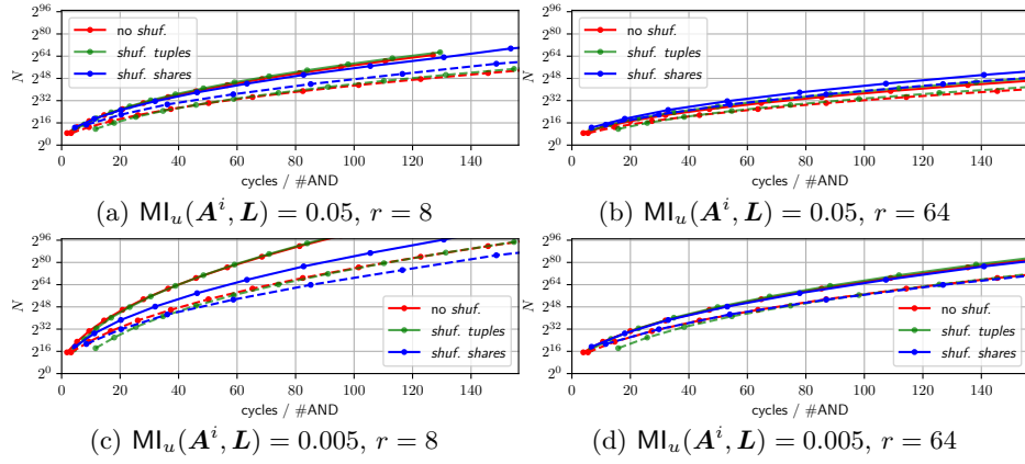
Figure 9: Cycles vs. security for 128 bitwise ANDs for various noise levels and randomness cost. Continuous are for bs = 32 and dashed ones for bs = 16 . The leftmost bullets stand for d = 2 and the value of d is increased by one for each step of the curves.
