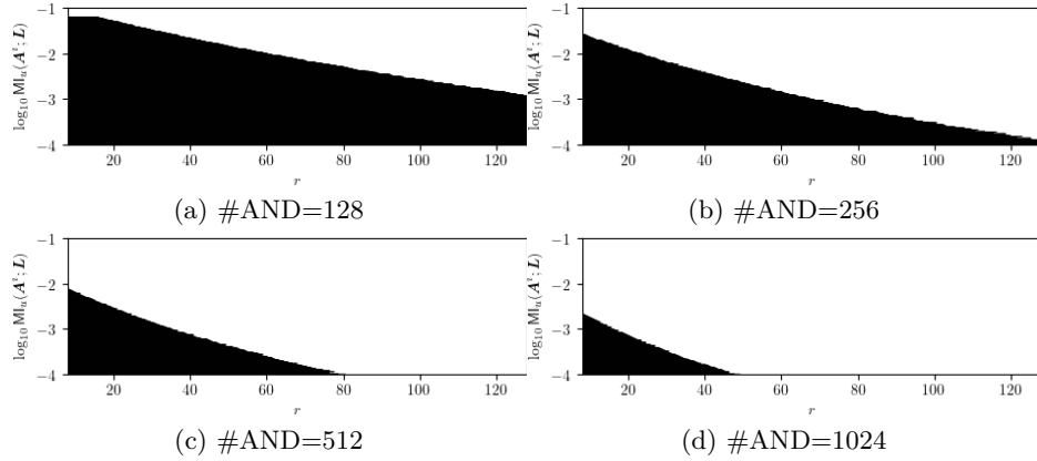
Figure 11: Masking + shuffling shares design space for a 64-bit security target and bs = 32 . Masking only is the more efficient than masking + shuffling in black areas.
