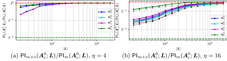
Figure 13: Information loss per share between shuffled + masked and masked only implementations PI_{m+s}(A_c^0; L)/PI_m(A_c^0; L) in function of the # of dimensions exploited.
