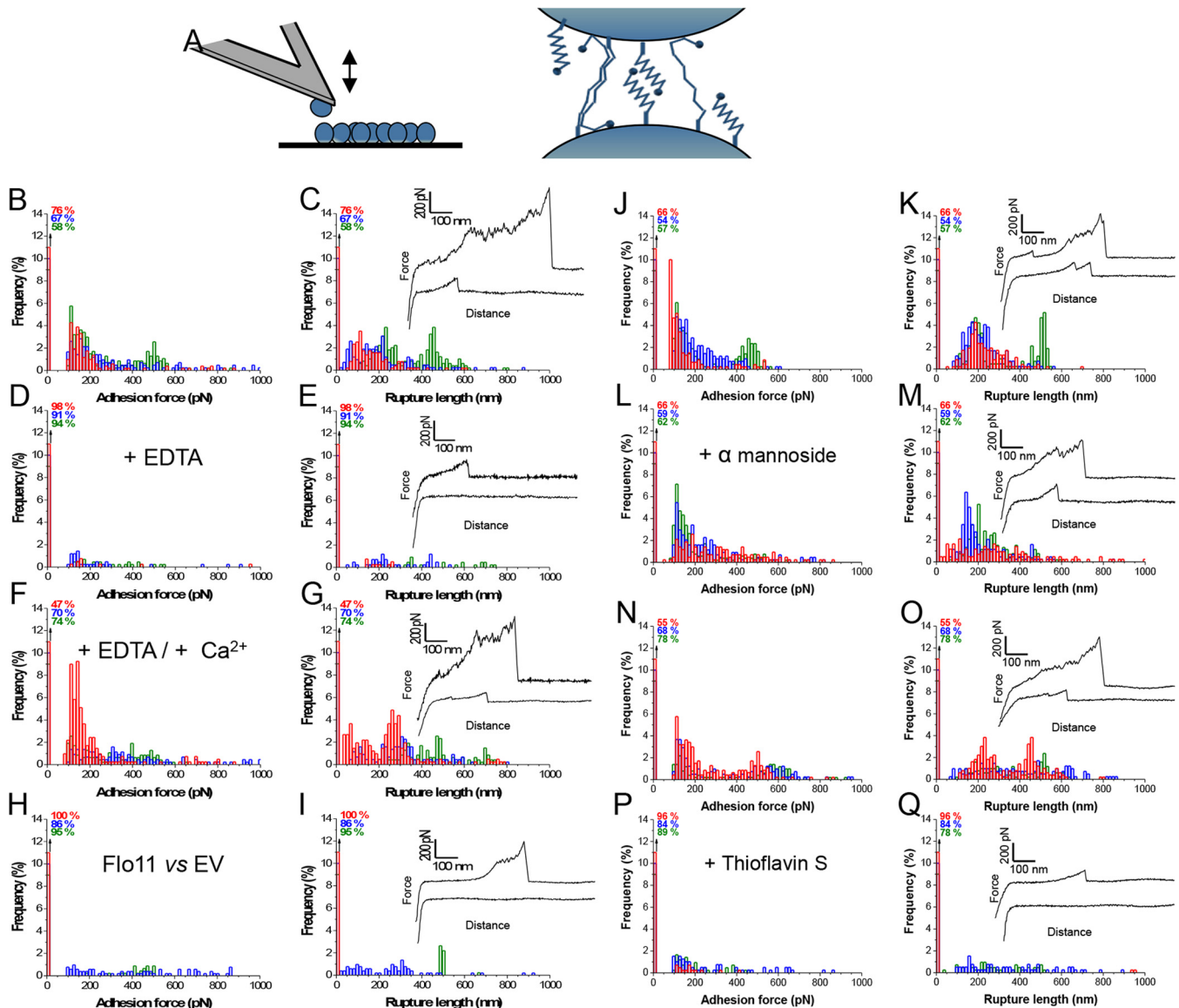
FIG 7 Forces in Flo11p-mediated cell-cell adhesion. (A) Principle of single-cell force spectroscopy. (Left) Single yeast cells were attached to a polydopamine-coated tipless cantilever, and curves of force between cell probes and yeast aggregates were acquired. (Right) Cartoon of homotypic interactions of the flocculins. Shown are adhesion force histograms (B, D, F, H, J, L, N, P) and rupture length histograms (C, E, G, I, K, M, O, Q) with representative force curves obtained by recording multiple force-distance curves for Flo11p-expressing cells in acetate buffer containing 200 \mu\text{M} \text{CaCl}_2 (B, C) or after the addition of 10 mM EDTA (D, E) and further addition of 400 \mu\text{M} \text{CaCl}_2 (F, G). (H, I) Force data obtained with Flo11p-expressing cells and yeast cells expressing no flocculin (EV). (L, M) Effects of methyl \alpha -D-mannopyranoside at 40 mg/ml added to the buffer in the experiments shown in panels J and K. For those shown in panels P and Q, 200 \mu\text{M} ThS was added to the cells shown in panels N and O. Red, blue, and green represent results from three different cell pairs from independent cultures ( n = >400 curves for each cell). All curves were obtained at 20°C by a constant approach at a retraction speed of 1 \mu\text{m} \cdot \text{s}^{-1} with a 1-s contact time.
