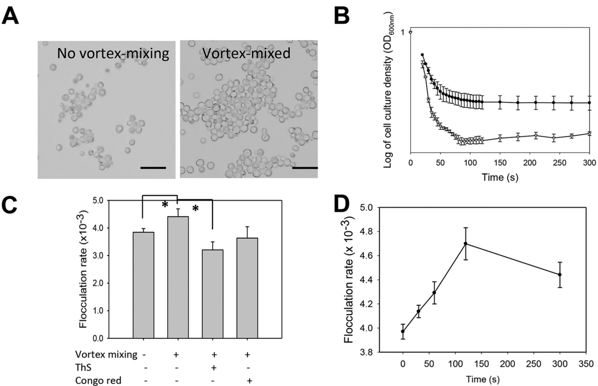
FIG 3 Effects of vortex mixing on the flocculation of S. cerevisiae cells expressing Flo1p. (A) Cells were left untouched or vortex mixed and then visualized in the absence of Ca 2+ . Scale bars = 20 \mu m. (B) Flocculation assays after the addition of 1.0 mM Ca 2+ . Cells were not mixed (●) or vortex mixed for 5 min (▽). (C) Flocculation rates in the absence or presence of the inhibitors ThS (200 \mu M) and CR (0.5 mM) ( n = 3 ). *, P < 0.01 (Student's t test). (D) Effect of duration of vortex mixing on activation of flocculation.
