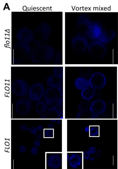
FIG 5 ThT fluorescence on the surface of Flo11p- and Flo1p-expressing S. cerevisiae . Shown are fluorescence confocal micrographs of cells under quiescent and vortex-mixed conditions taken right after vortex mixing as described in Materials and Methods and then stained with 500 nM ThT. Scale bars represent 5 \mu m. The boxed cells are further enlarged in the insets.
