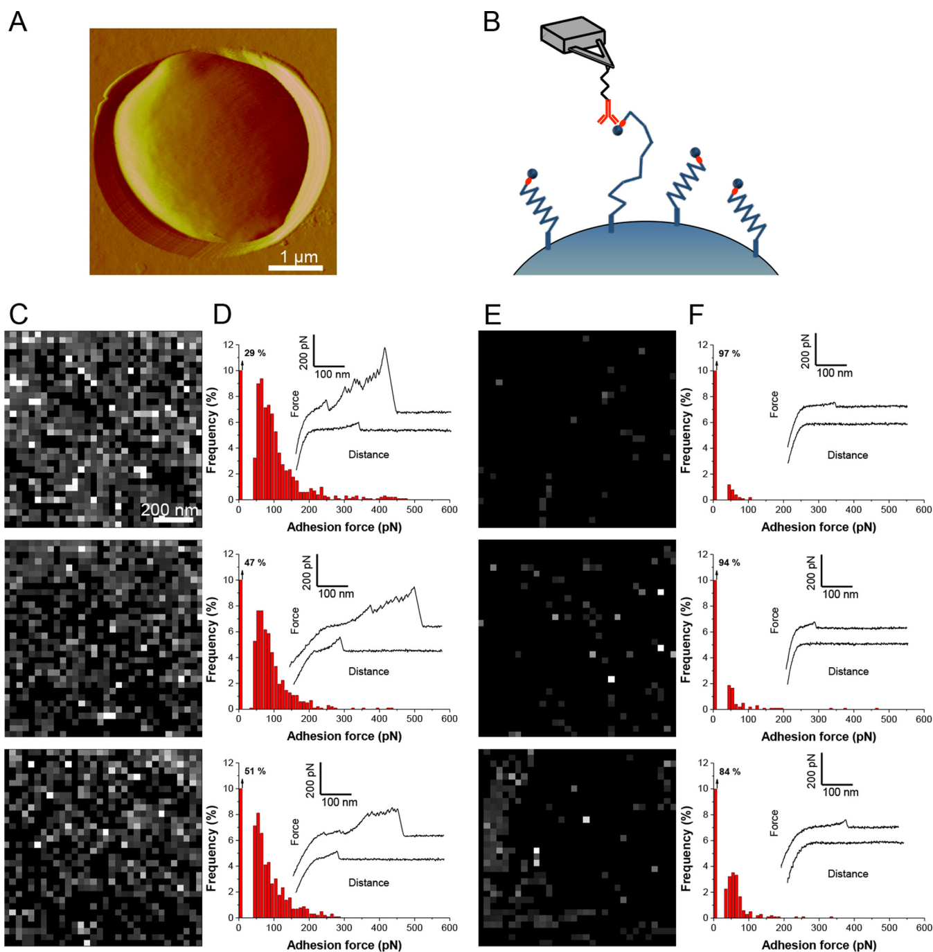
FIG 6 Single-molecule imaging of V5-Flo11p proteins on yeast cells. (A) AFM deflection image recorded in buffer, showing an S. cerevisiae cell expressing V5-tagged Flo11p proteins trapped in a porous membrane for AFM analysis. (B) Single-molecule detection of V5-tagged Flo11p proteins with anti-V5 antibody-coated AFM tips. (C to F) Adhesion force maps (1 by 1 μm) (C, E) and adhesion force histograms ( n = 1,024 curves) (D, F), with representative force curves, obtained in buffer between anti-V5 tips and three different yeast cells expressing V5-tagged Flo11p (C, D) or no flocculin (E, F) (different cultures and different tips). Pixels are shaded according to the rupture force necessary to disrupt binding, with no binding depicted as black and strong interactions shown as white.
