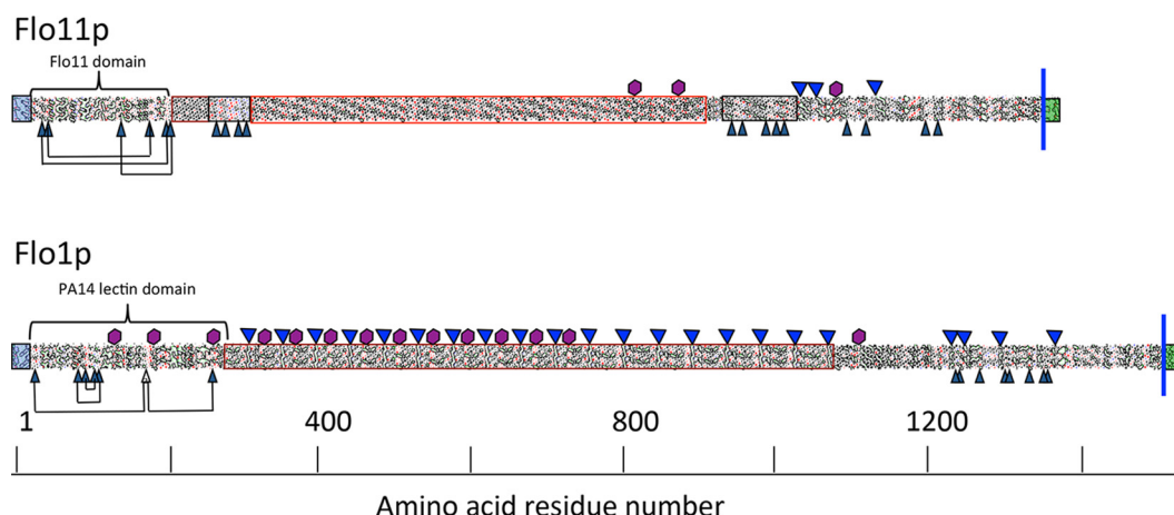
FIG 1 Primary-structure analyses of Flo1p and Flo11p. Hydrophobic-cluster analyses highlight domain structure and patterns of repeats (15). Secretion signal sequences are boxed in blue, C-terminal GPI addition signals are boxed in green, and the blue line denotes the position of GPI signal cleavage and anchorage to cell wall glucan (13). Central repeat regions are in unshaded boxes. Cys residues are black arrowheads, with disulfides marked where they have been mapped in the N-terminal domains (12). Potential N-glycosylation sites are marked with purple hexagons, and sequences with a \beta -aggregation potential of >30\% in TANGO are marked with blue triangles (21).
