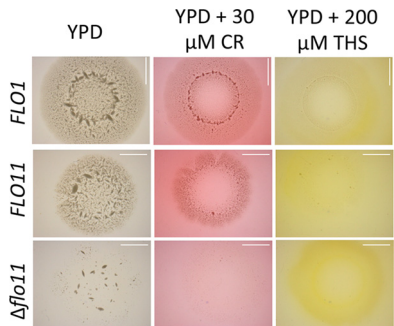
FIG 4 Agar invasion assays. Cells were grown on YPD plates for 2 weeks with or without amyloidophilic dyes and then washed and imaged from the bottom of the petri plate. Concentrations: CR, 30 \mu M; ThS, 200 \mu M. Scale bars represent 5 mm.
