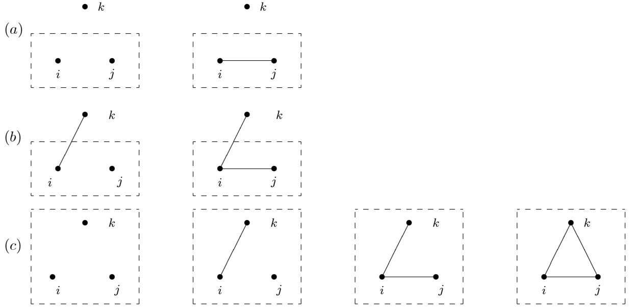
Figure 5: Contractually Stable coalitional networks in the RD model
