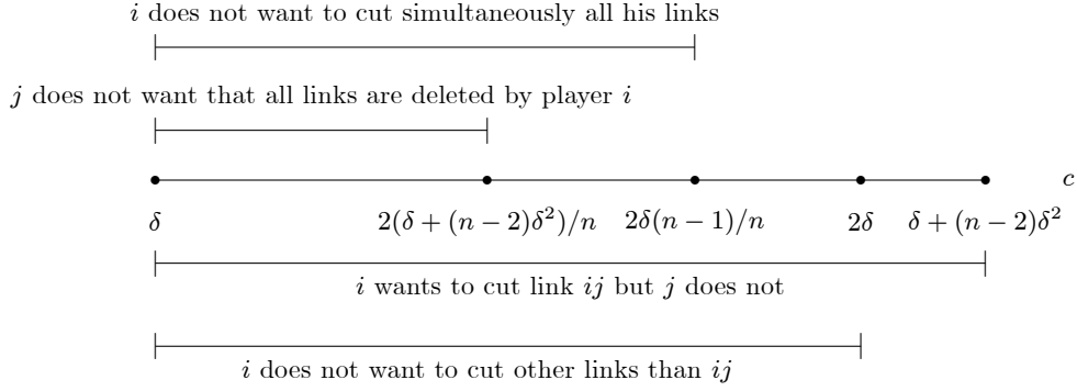
Figure 4: Incentives for deleting links in the star network
