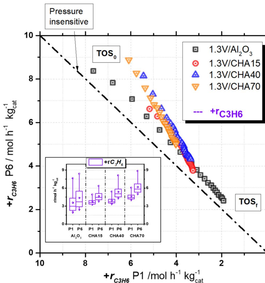
Fig. 3 . Pressure effect over V supported on \text{Al}_2\text{O}_3 , CHA15, CHA40 and CHA70 zeolites with a nominal load of 1.3 \text{ mmol} \cdot \text{g}_{\text{support}}^{-1} . The analysis shows propylene produced at P1 = 1 \text{ barg} (X-axis) and P6 = 6 \text{ barg} (Y-axis). A pressure insensitive diagonal is shown as a dashed line. \text{TOS}_0=0 and \text{TOS}_f=200 \text{ min} . small inset is propylene production rate, all of them for 1 and 6 barg displayed by box and whisker analysis. Reaction Conditions: 600^\circ\text{C} using gas ratios of \text{CO}_2/\text{C}_3\text{H}_8/\text{Ar}/\text{N}_2 = 2.5/2.5/47.5/47.5 \text{ Nml} \cdot \text{min}^{-1} , GHSV 3.0 \times 10^4 \text{ Nml} \cdot \text{gas} \cdot \text{mlcat}^{-1} \cdot \text{h}^{-1} , and WHSV 1.5 \text{ gC}_3\text{H}_8 \cdot \text{gcat}^{-1} \cdot \text{h}^{-1} . The effect of slightly varying GC sampling times was corrected through interpolation of the experimental data. The total time on stream (TOS) duration was 200 minutes, with product sampling conducted every 10 minutes. See Fig.S13 pressure effect over propane consumption rate, \text{CO}_2 consumption rate and propylene production.
