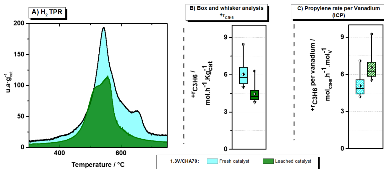
Fig. 9. Vanadium Leaching treatment over 1.3V/CHA70. A) \text{H}_2 -TPR profile before (fresh) and after leaching; B) Box-and-whisker analysis for both leached and fresh catalysts C) Box-and-whisker analysis for both leached and fresh catalysts, showing normalized propylene production per mole of vanadium. Reaction at 600^\circ\text{C} for 200.0(2) mg catalyst using gas ratios of \text{CO}_2/\text{C}_3\text{H}_8/\text{Ar}/\text{N}_2 = 2.5/2.5/47.5/47.5 \text{ Nml} \cdot \text{min}^{-1} , and WHSV 1.5 \text{ g}_{\text{C}_3\text{H}_8} \text{ g}_{\text{cat}}^{-1} \text{ h}^{-1} . The total time on stream (TOS) duration was 200 minutes, with product sampling conducted every 10 minutes.
