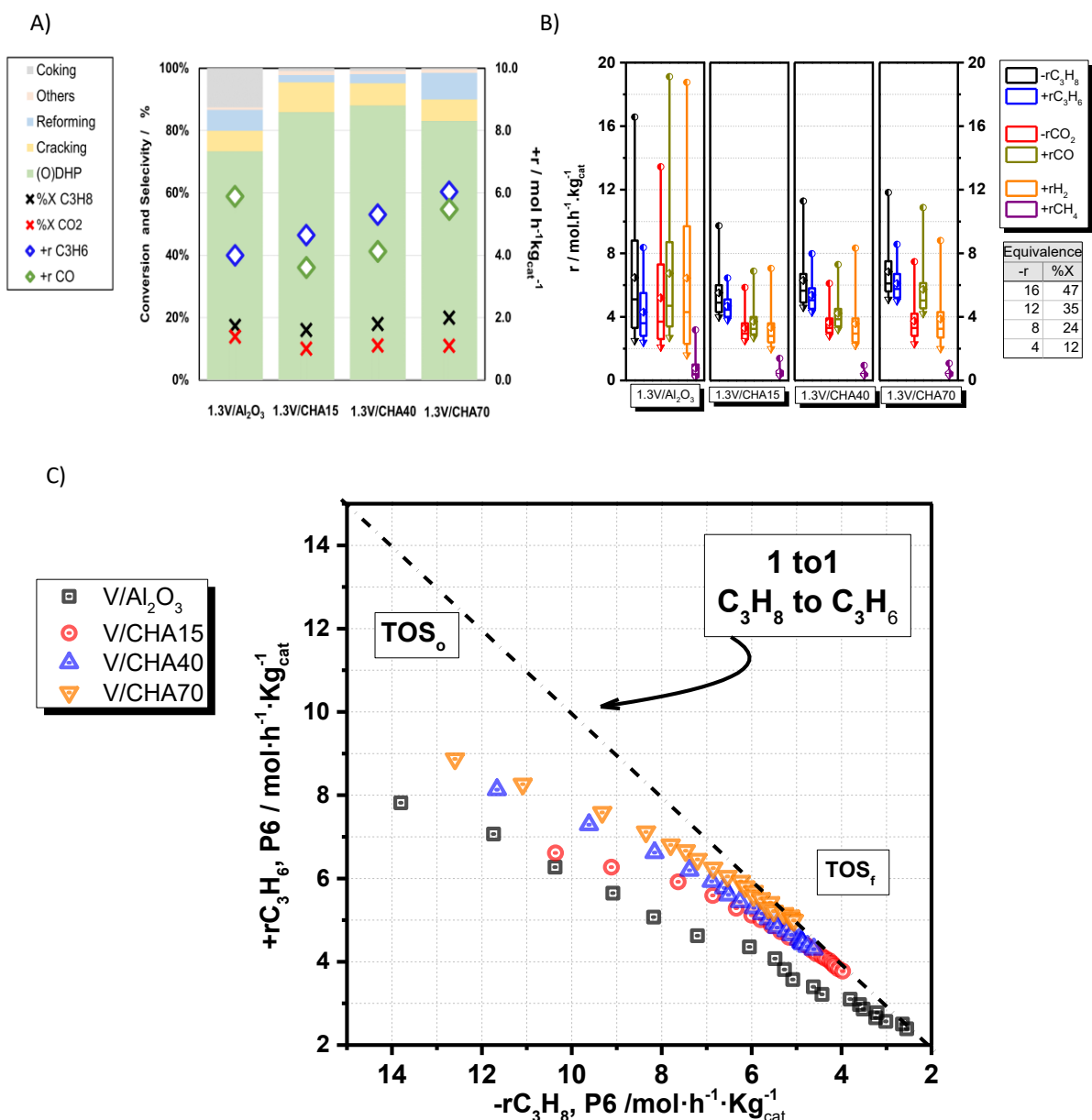
Fig. 2 A) Conversion and selectivity (left axis) and product rates (right axis) averaged during TOS stage reactions over 1.3V/Al 2 O 3 , 1.3V/CHA15, 1.3V/CHA40, and 1.3V/CHA70. B) Box and whisker analysis for ODHP reactions over 1.3V/Al 2 O 3 , 1.3V/CHA15, 1.3V/CHA40, and 1.3V/CHA70. Small inset displays the equivalence between reactant rate consumed and approximate conversion. C) Propylene production vs propane consumption rates. Reactions were performed at 600 °C under 6 barg pressure and gas ratios of CO 2 /C 3 H 8 /Ar/N 2 = 2.5/2.5/47.5/47.5 Nml min -1 , WHSV 1.5 g C 3 H 8 g cat -1 h -1 . The total time on stream (TOS) duration was 200 minutes, with product sampling conducted every 10 minutes. Subscripts o and f in TOS indicate the profile at time zero and 200 min respectively.
