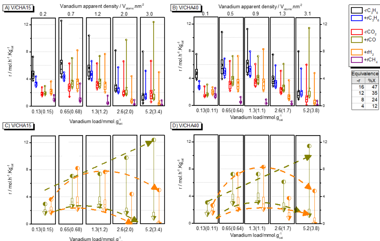
Fig. 4 Impact of vanadium load on the catalytic performance across two CHA supports. (A, B): Catalytic performance study based on reactants consumption and production molar rates. Dual X-axis. Bottom X-axis: nominal load (ICP measured load). Top X-axis: Vanadium apparent density. Small inset displays the equivalence between reactant rate consumed and approximate conversion. (C, D) Separate plots highlighting the extreme points (initial and final catalytic profiles) catalytic profile for CO and H 2 production. Reaction at 600 °C using gas ratios of CO 2 /C 3 H 8 /Ar/N 2 = 2.5/2.5/47.5/47.5 Nml·min -1 , GHSV 3.0E+4 Nml·gas mlcat -1 h -1 , and WHSV 1.5 gC 3 H 8 gcat -1 h -1 . For further details, refer to Supplementary Material Fig. S8-S11. The total time on stream (TOS) duration was 200 minutes, with product sampling conducted every 10 minutes.
