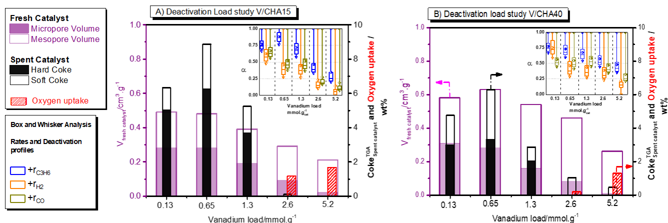
Fig. 5 Impact of Vanadium load on the catalytic performance across two CHA supports. (A, B): Assessment of fresh textural properties and comparative deactivation analysis: Purple bars and left axis are pore volume by \text{N}_2 physisorption. Black and with bars represent coke. Soft coke is the weight loss between 200 °C and 600 °C under a nitrogen atmosphere, and hard coke determinate shifting at 600 °C to air. Small inset square: box and whisker plots to illustrate deactivation profiles evaluating the residual activity \alpha (where 1 is the initial activity and 0 correlates with total deactivation). Reaction at 600 °C using gas ratios of \text{CO}_2/\text{C}_3\text{H}_8/\text{Ar}/\text{N}_2 = 2.5/2.5/47.5/47.5 \text{Nml}\cdot\text{min}^{-1} , GHSV 3.0\text{E}+4 \text{Nml}\cdot\text{gas}\cdot\text{mlcat}^{-1}\cdot\text{h}^{-1} , and WHSV 1.5\text{ gC}_3\text{H}_8\cdot\text{gcat}^{-1}\cdot\text{h}^{-1} . For further details, refer to Fig. S15 and Fig. S22.
