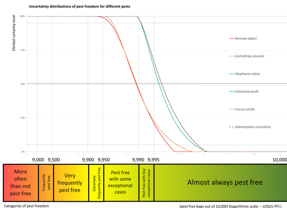
Figure 4: Elicited certainty (y-axis) of the number of pest-free J. polyanthum bags (x-axis; log-scaled) out of 10,000 bags designated for export to the EU introduced from Uganda for all evaluated pests visualised as descending distribution function. Horizontal lines indicate the percentiles (starting from the bottom 5%, 25%, 50%, 75%, 95%)
