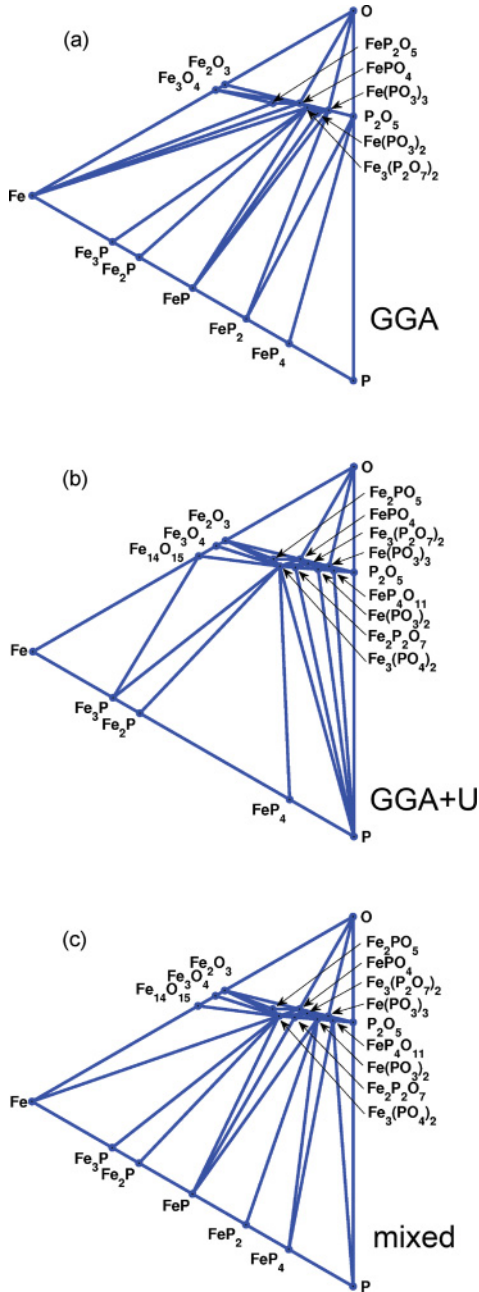
FIG. 5. (Color online) Computed 0 K, 0 atm phase diagram of the Fe-P-O system within the (a) GGA methodology, (b) GGA + U methodology, and (c) mixed GGA/GGA + U technique of the current work. The GGA phase diagram fails to reproduce known phases in the Fe-O and Fe-P-O composition ranges, whereas the GGA + U methodology fails along the Fe-P line. Only the mixed GGA/GGA + U phase diagram of the current work successfully reproduces known phases in all composition areas.
