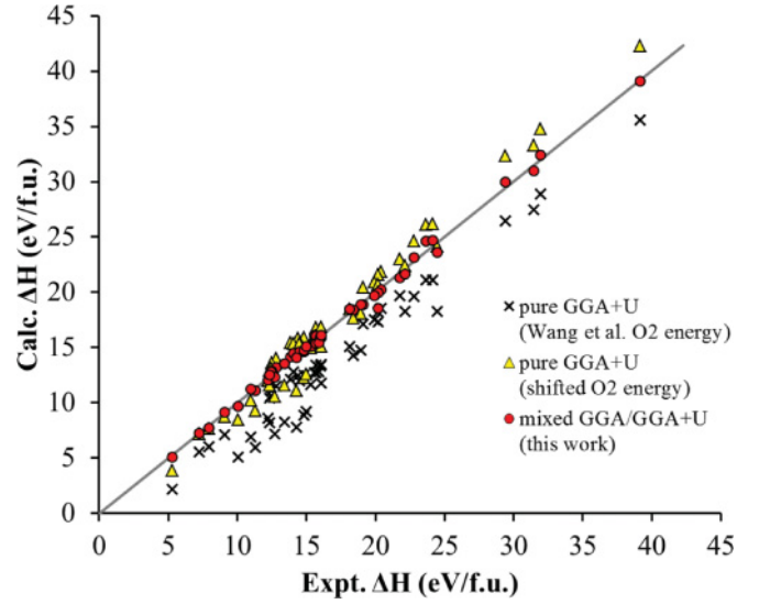
FIG. 3. (Color online) Computed and experimental formation enthalpies of ternary oxides from the elements using (a) GGA + U for all compounds with Wang’s \text{O}_2 correction, (b) GGA + U with an \text{O}_2 correction fitted to minimize the MARE, and (c) the mixed GGA/GGA + U framework proposed in this paper. The mixed GGA/GGA + U framework best reproduces experimental results while retaining an \text{O}_2 energy consistent with GGA calculations. The full list of compounds and results can be found in the Appendix.
