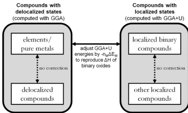
FIG. 1. (Color online) Calculation methodology for mixing GGA and GGA + U calculations. The elements and all delocalized/unrelated compounds are computed with GGA. We compute with GGA + U all localized compounds; in this work, this includes any oxide containing one of the elements listed in Table I. Other types of localized compounds, such as transition metal sulfides or fluorides, might also fall within the realm of GGA + U calculation. The energy adjustment applied to GGA + U can be envisioned as a virtual reaction between the elements and localized binary compounds that is determined using experimental data. This energy adjustment is described in Eq. (6); details are provided in the surrounding text.
