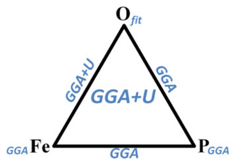
FIG. 4. (Color online) Strategy for generating the Fe-P-O phase diagram using a mixture of GGA and GGA + U calculations. Regions of the phase diagram containing both Fe and O are computed with GGA + U , whereas the remaining regions are computed with GGA . This strategy follows the more general guidelines outlined in Fig. 1. The O_2 energy is taken from Wang et al. 's fit. 15
