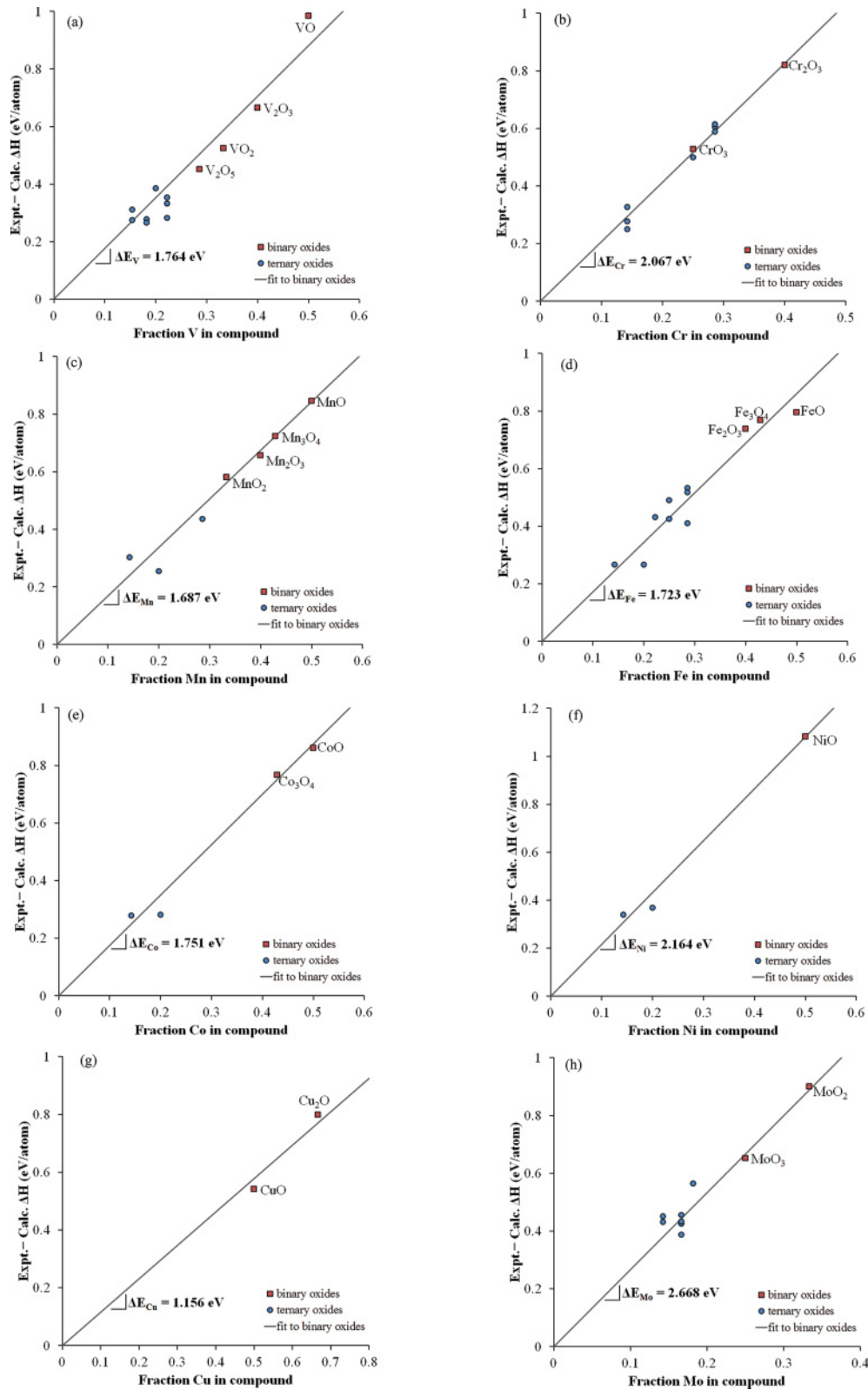
FIG. 2. (Color online) Differences between experimental and calculated and formation enthalpies as a function of metal content for V, Cr, Mn, Fe, Co, Ni, Cu, and Mo. The calculations used GGA for the metals and GGA + U for the binary and ternary oxides. The differences from experiment increase linearly with metal content in the oxides; this difference can be removed simply by adjusting GGA + U energies for the oxides via Eq. (6). The gray line is fitted via least-squares to the binary-oxide data alone (red squares), and its slope represents the magnitude of the adjustment \Delta E_M , which is specific to the metal and U value. However, ternary oxides are also well represented by this line, suggesting that the adjustment generalizes beyond the binary oxides.
