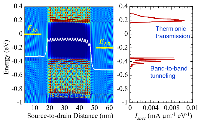
FIG. 3. (Left panel) Local Density of States in the GNM device with E_G = 508 meV for V_{GS} = 0.1 V and V_{DS} = 0.2 V corresponding to a Dirac point of the transfer characteristics. The source and drain Fermi levels E_{FS} and E_{FD} are indicated and the potential profile at the neutrality point is superimposed. (right panel) Corresponding energy spectrum of current.
