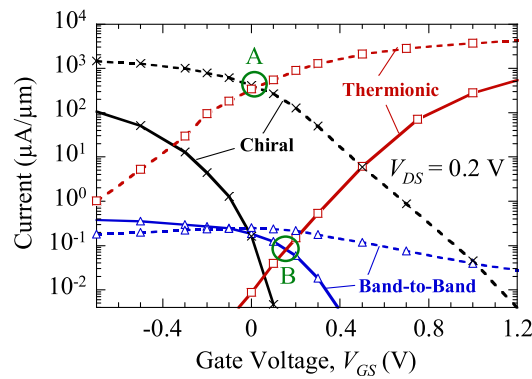
FIG. 2. The different contributions to the current in pristine (dashed lines) and GNM (solid lines) transistors as a function of the gate voltage, for the drain voltage V_{DS} = 0.2 V. In the latter case, the GNM lattice bandgap is equal to 508 meV.
