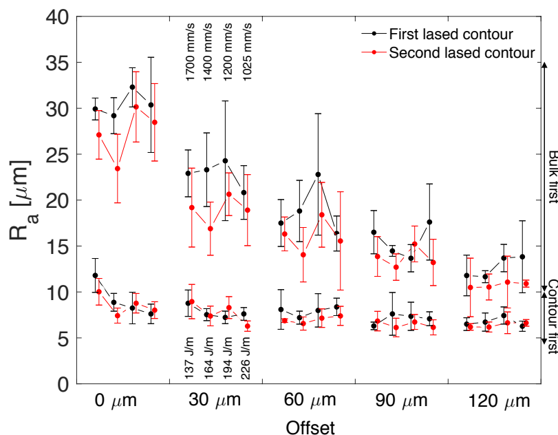
Figure 1. Roughness evolution as a function of the offset parameters, Scan speed and scan strategy.
