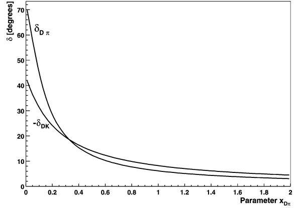
Fig. 1. Final state interaction phases in B \rightarrow D\pi and B \rightarrow DK as a function of the Regge variable x_{D\pi} defined in Eq. (7).
