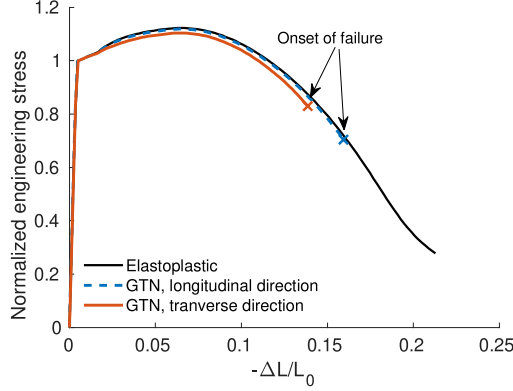
Figure 18: Comparison of the engineering stress/engineering strain response obtained with the elastoplastic model and with the GTN model in the longitudinal and transverse directions.
