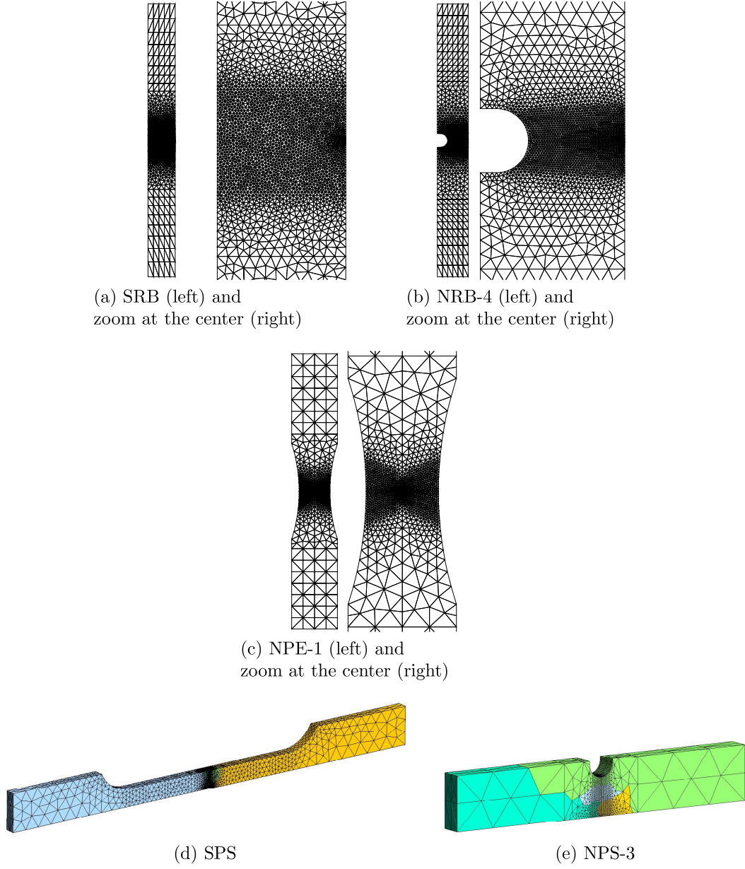
Figure 14: Finite element meshes considered in the elastoplastic simulations: (a) SRB specimen, (b) NRB-4 specimen, (c) NPE-1 specimen, (d) SPS specimen, and (e) NPS-3 specimen.
