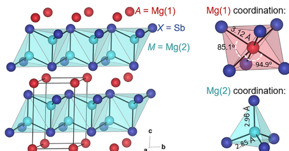
Figure 1. \text{CaAl}_2\text{Si}_2 Structure Type
