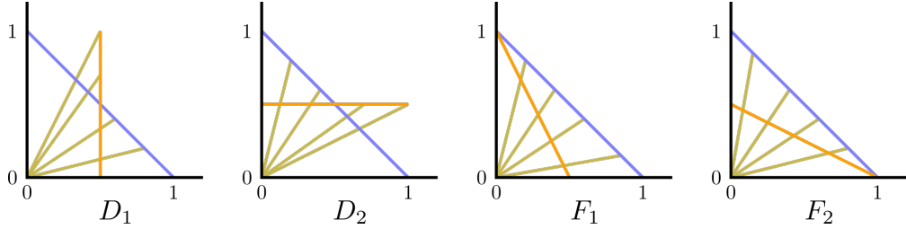
Figure 8: The four transformations of Corollary 16, corresponding to possible successful (D_1, D_2) and failed (F_1, F_2) message transmissions for 2 nodes. Points on the blue segment are moved to the orange segment using an affine transformation, then mapped along the yellow lines back to the blue line using a central projection from the origin.
