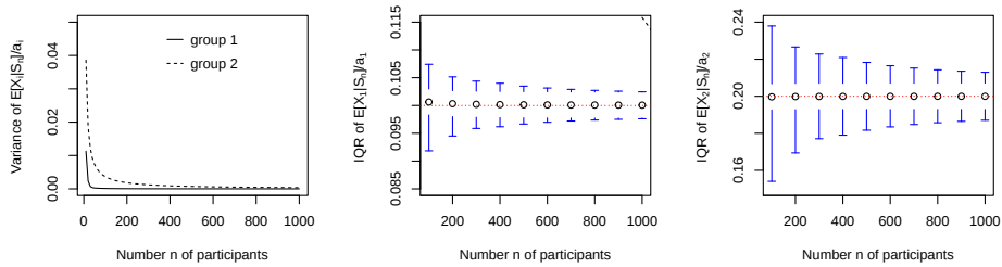
FIGURE 3. Variance of E[X_i|S_n]/a_i as a function of n \in \{10, 20, 30, \dots, 1000\} (left panel) for a participant in group 1 (continuous line) and in group 2 (broken line), median and interquartile range (IQR) of E[X_i|S_n]/a_i for n \in \{100, 200, 300, \dots, 1000\} in group 1 (middle panel) and in group 2 (right panel) for the pool described in Example 4.3. Horizontal lines in the central and right panels correspond to expected mortality credits.
