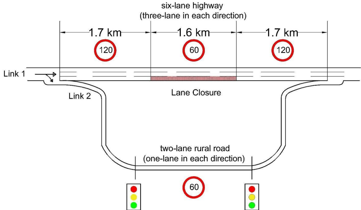
Figure 3: The simulation case study
