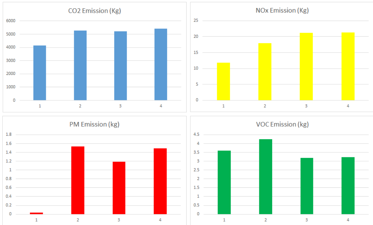
Figure 4: Exhausted emissions for different scenarios
