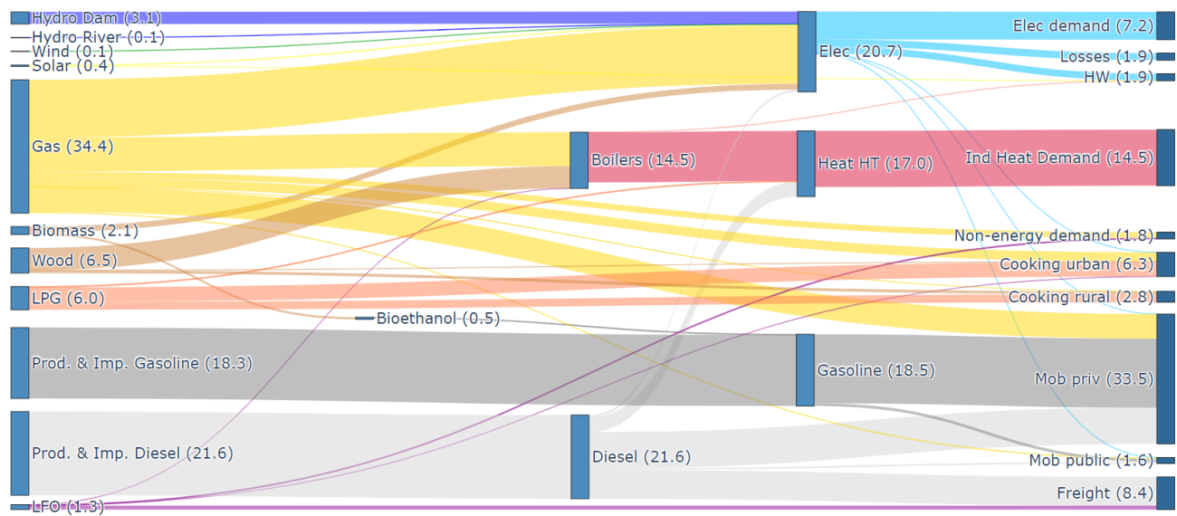
Figure 2: Energy flows of the modeled Bolivian energy system for 2021 (Units: TWh). The left side integrates all the resources while the right side retrieves the final energy consumption. The conversion technologies are in between. Energy exports are not represented. Abbreviations: mobility (mob), private (priv), electricity (Elec), liquefied petroleum gas (LPG), light fuel oil (LFO), industrial (Ind), domestic hot water (HW), low temperature (LT), high temperature (HT), importation (Imp), production (Prod).
