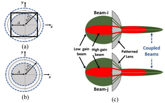
Fig. 2. Square (a) and circle-shaped (b) averaging surfaces for PD extractions of Gaussian beams. Patterned lens with distributed gain beams (c).
