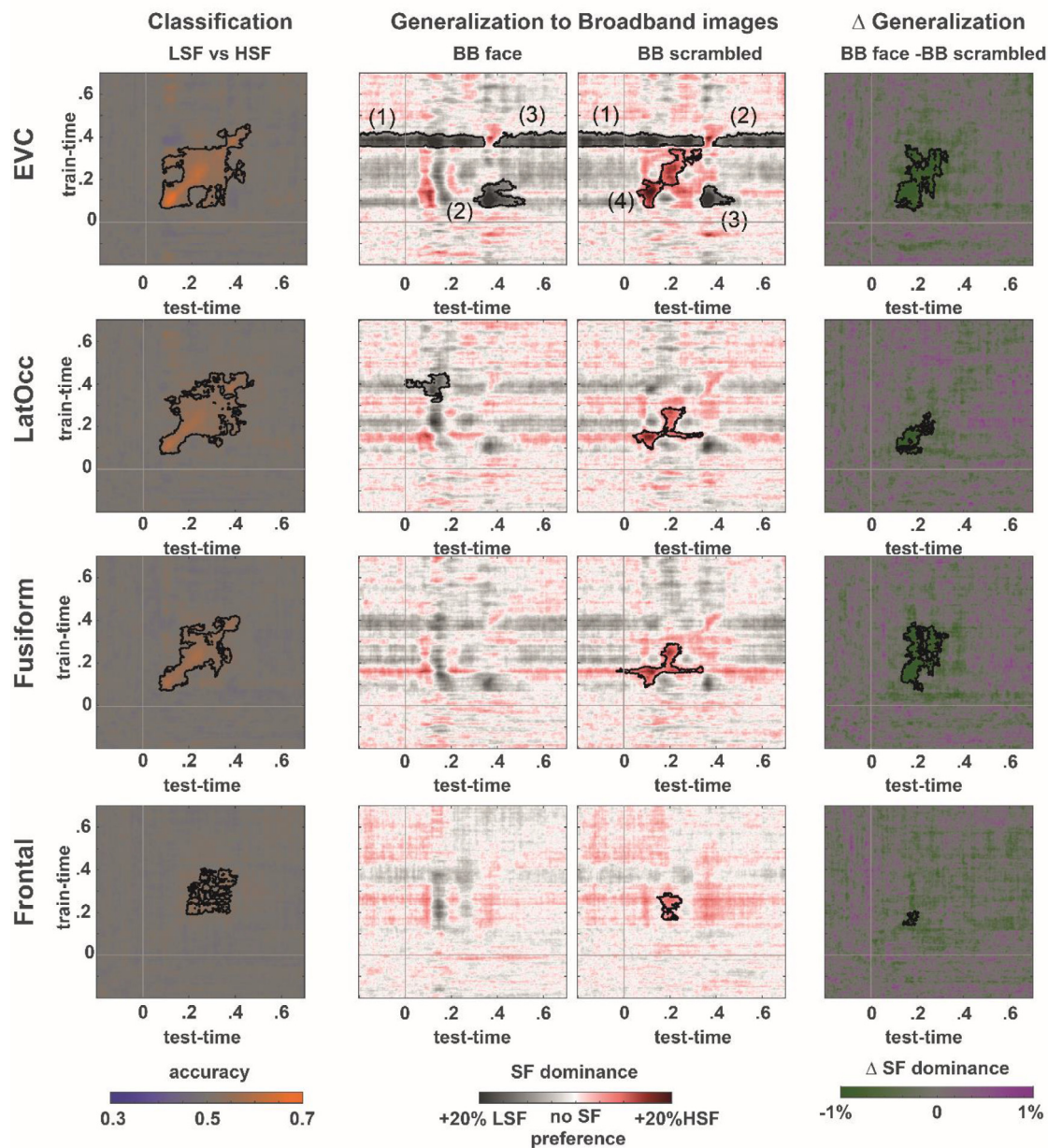
Fig. 5. Spatial frequency classification and generalization in source-space. All four ROI contain sufficient information to differentiate between scrambled LSF and HSF trials, although accuracies and latencies of successful classification differ substantially across them. When applying the classifiers trained on LSF vs HSF scrambled image trials to broadband image trials, the early visual cortex ROI shows a similar SF dominance pattern as observed in sensor-space with stronger HSF dominance in response to scrambled, compared to intact face images. Cluster indices reflect order in ranked cluster statistic (see table 2 ).
